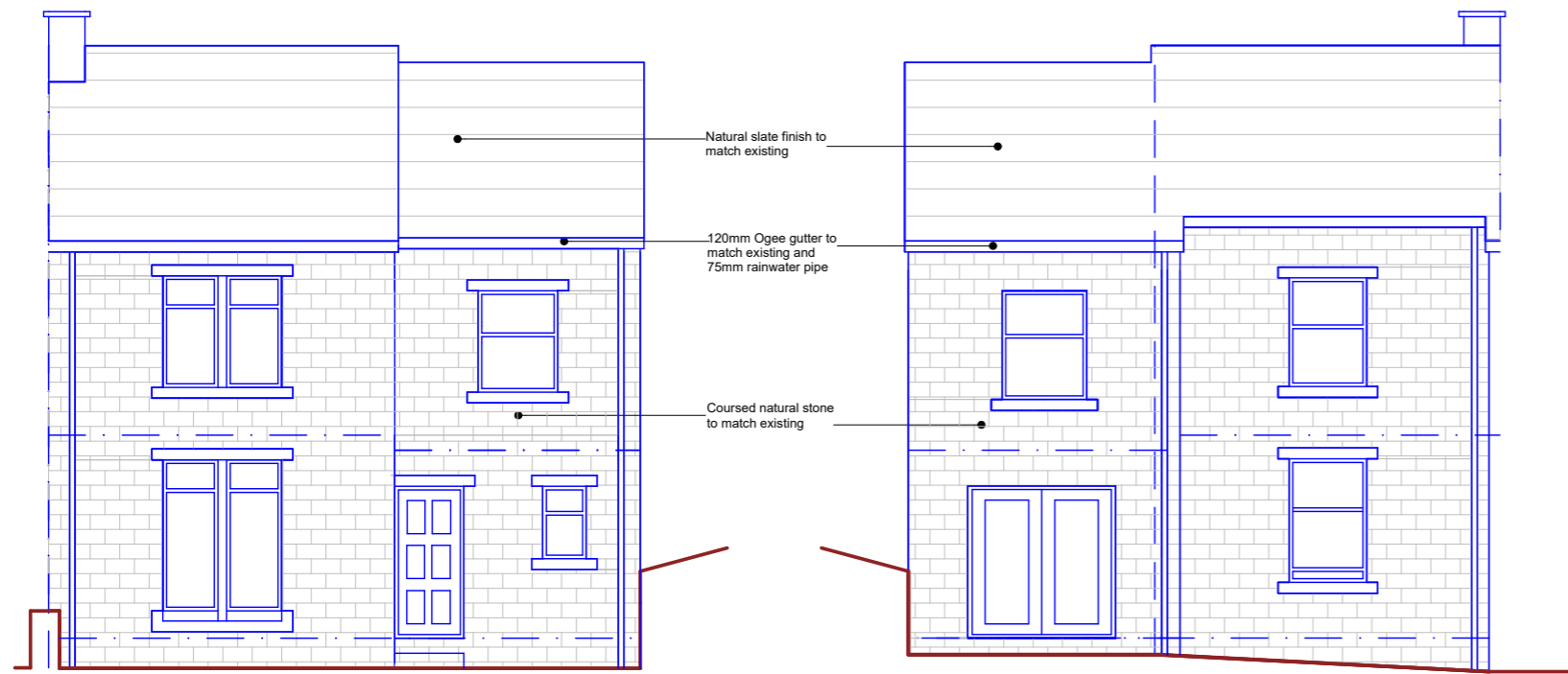
Front Elevation (East)
