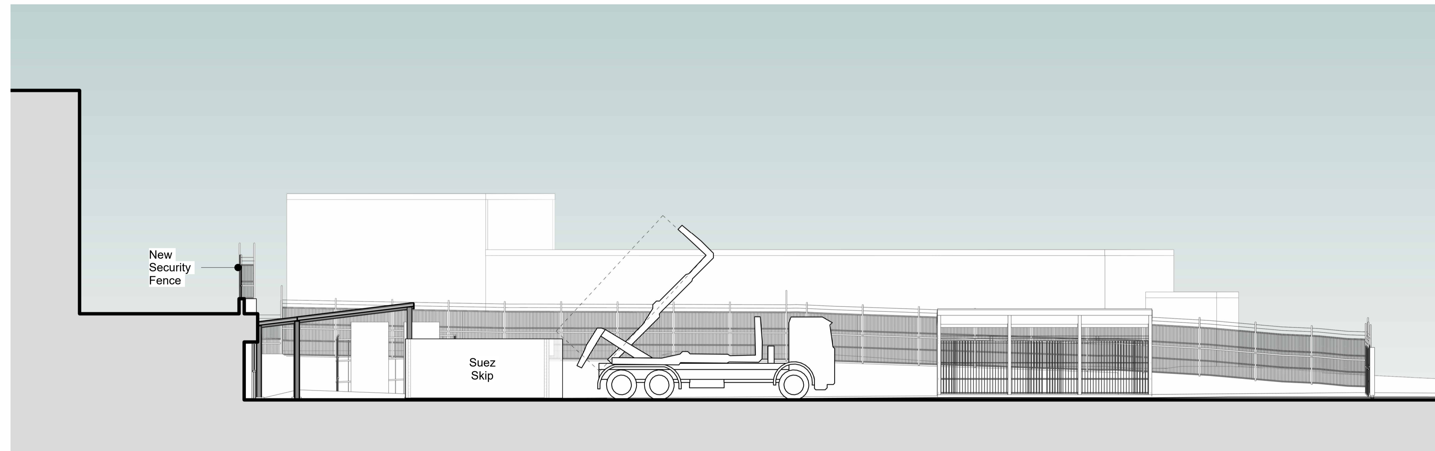
PROPOSED CANOPY SECTION A-A 1 : 100
