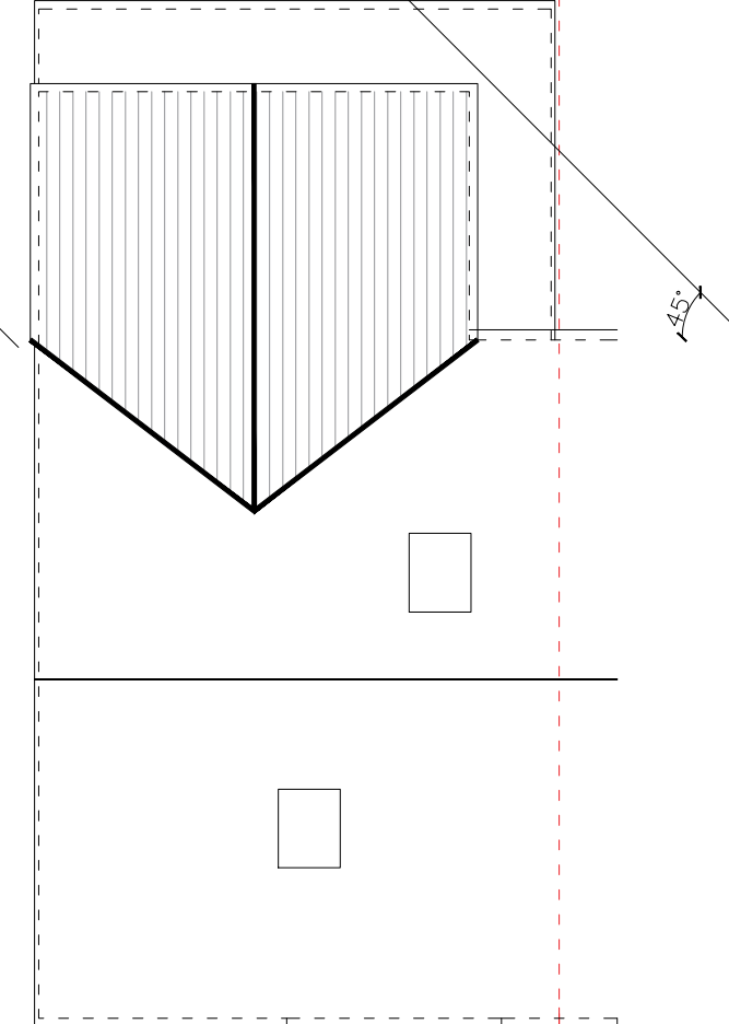
PROPOSED ROOF FLOOR PLAN
