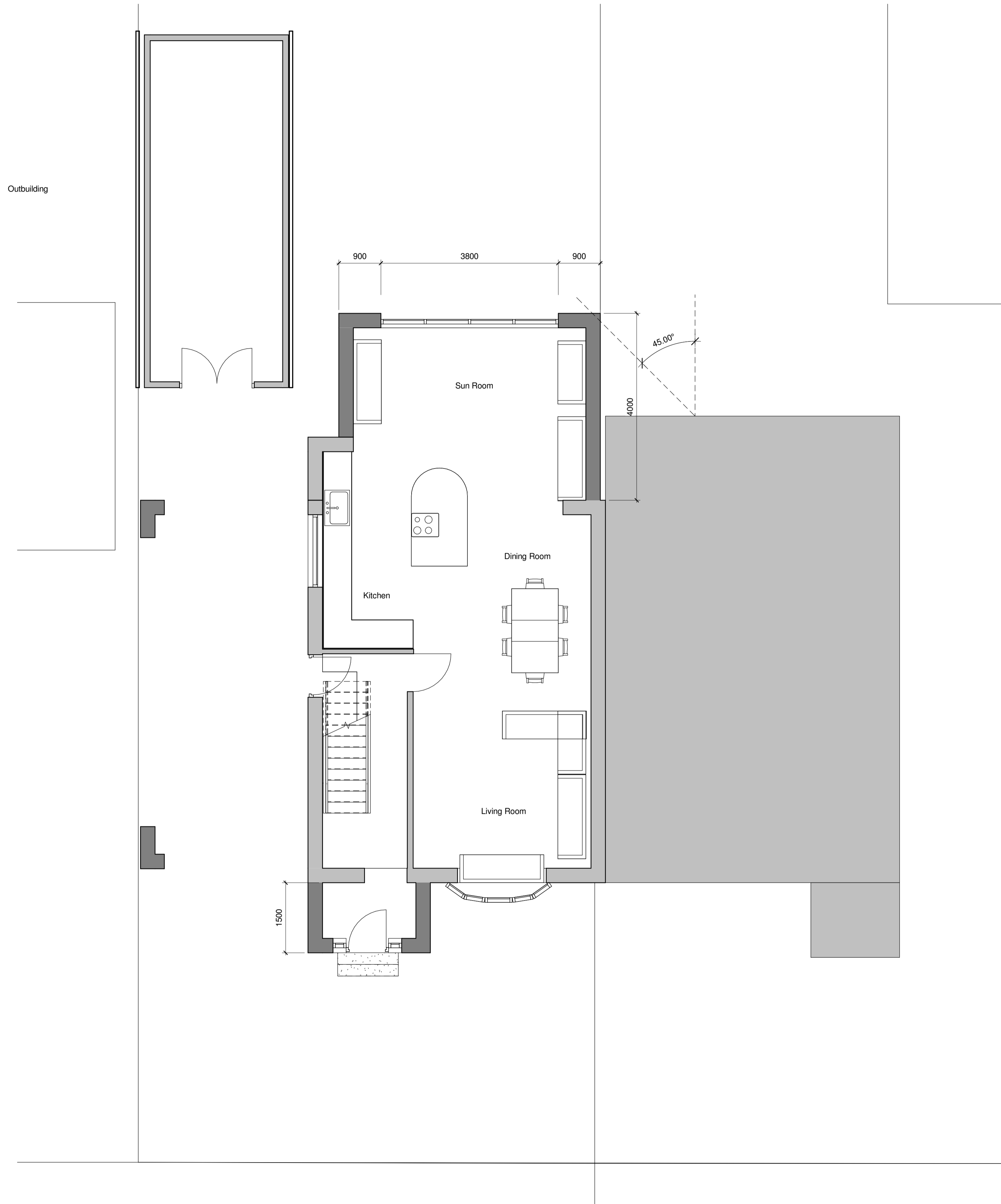
1 Proposed Level 0 Floor Plan 1 : 50
