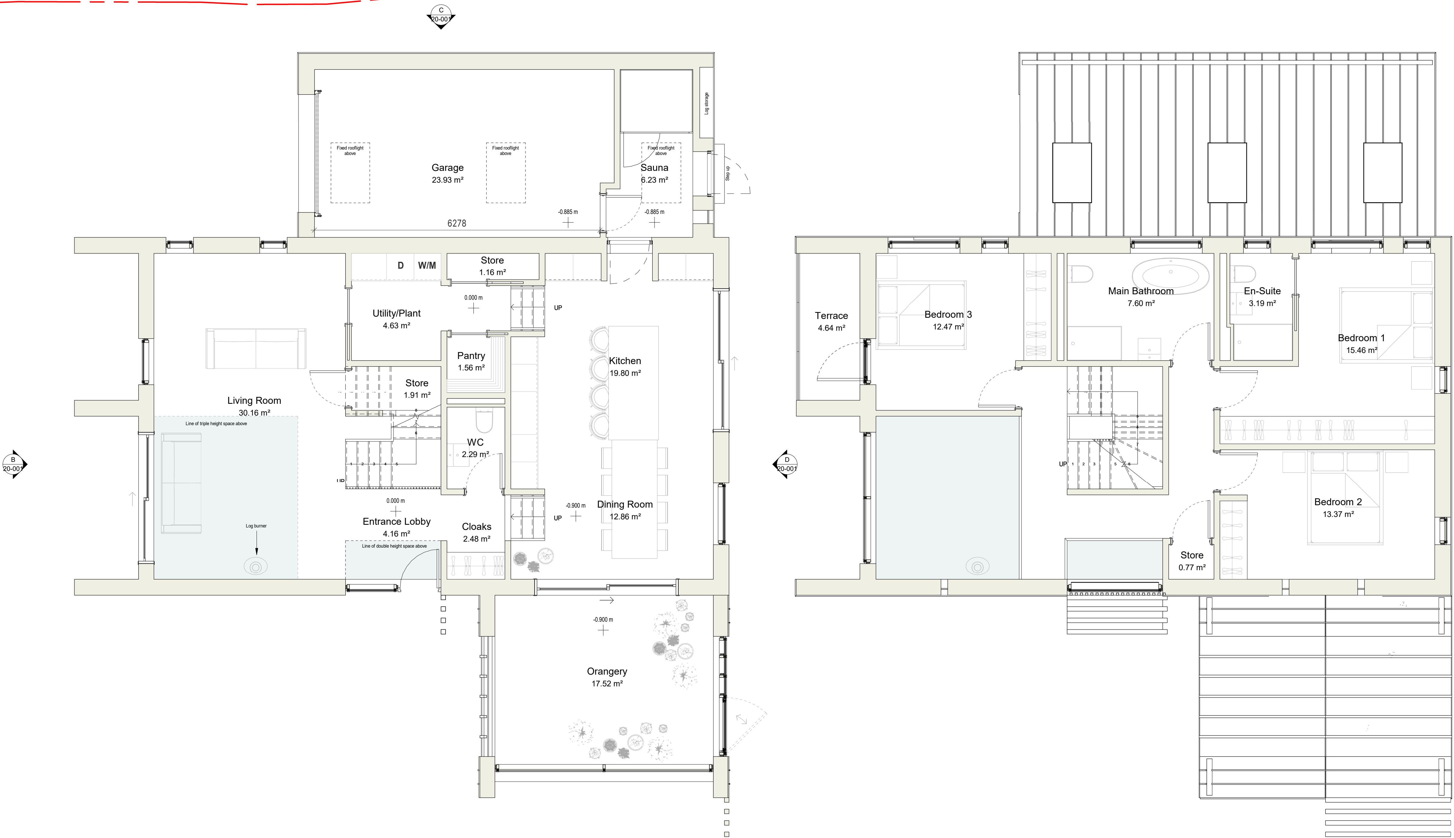
Ground Floor 1 : 50
