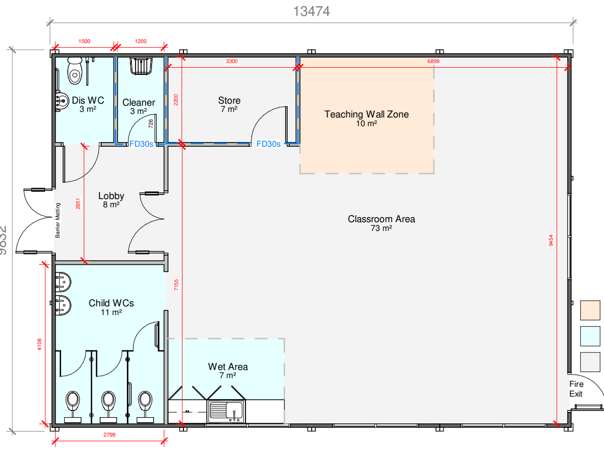
1 Proposed Layout 1 : 100
