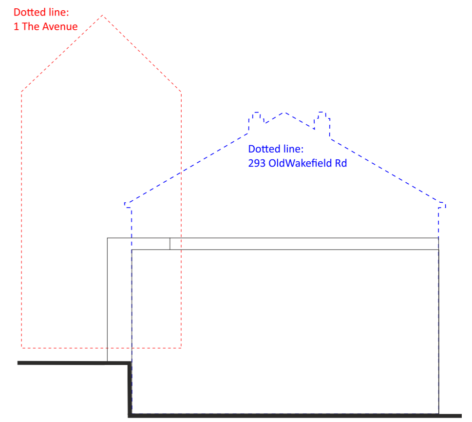
Existing South-West Elevation 'D' Scale 1:100
