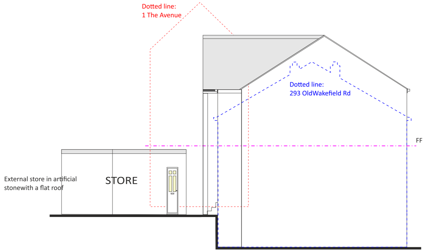
Proposed South-West Elevation 'D' Scale 1:100
