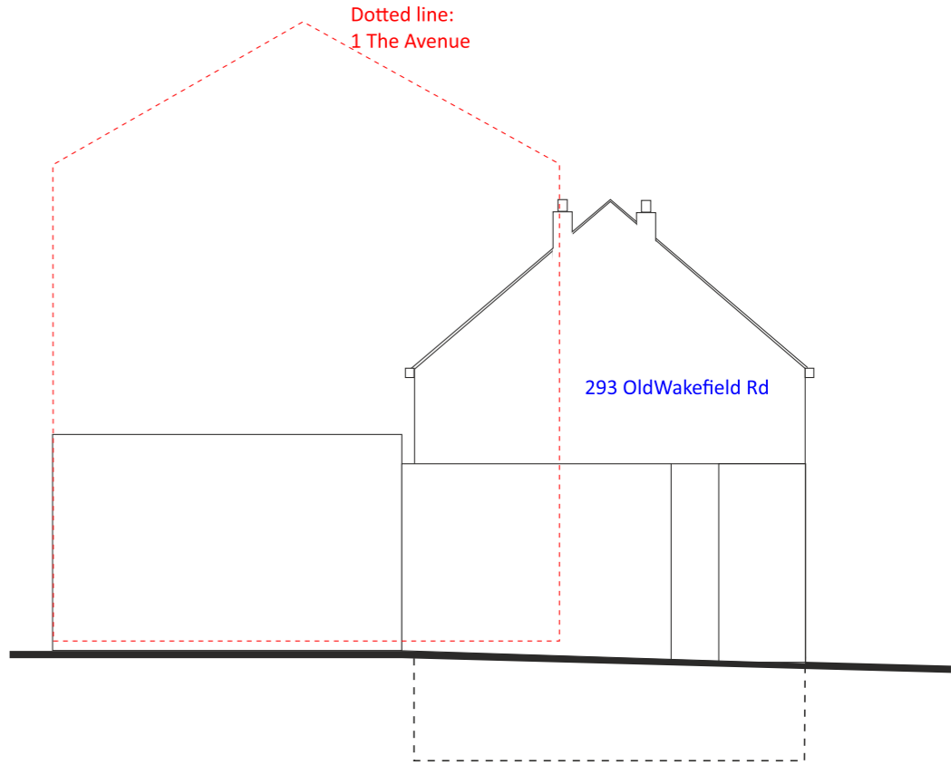
Existing North Elevation 'B' Scale 1:100
