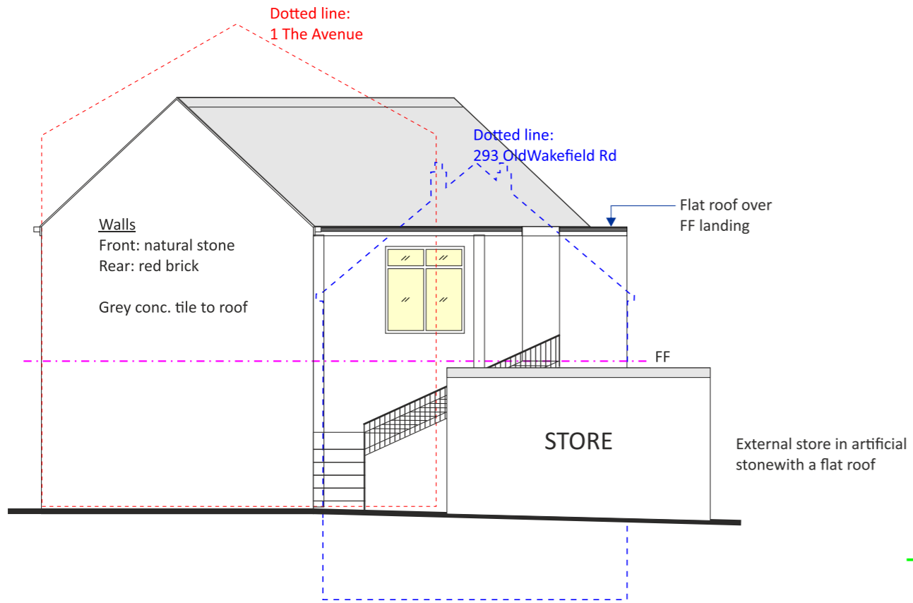
Proposed North Elevation 'B' Scale 1:100
