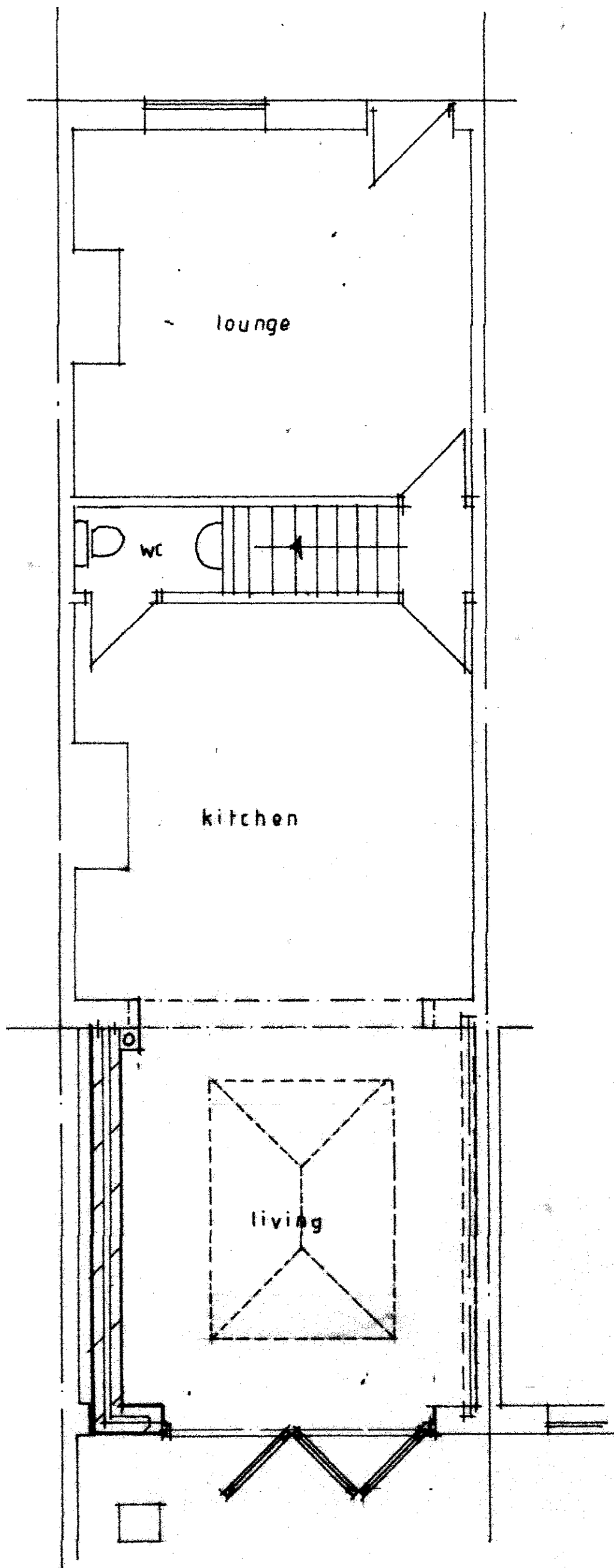
PROPOSED GROUND FLOOR PLAN SCALE 1:50 @ A3.
