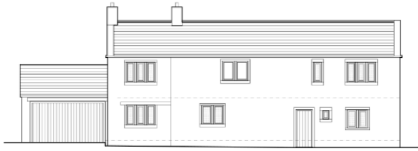
North Elevation 1:100
