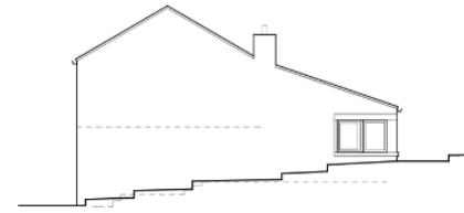
West Elevation 1:100
