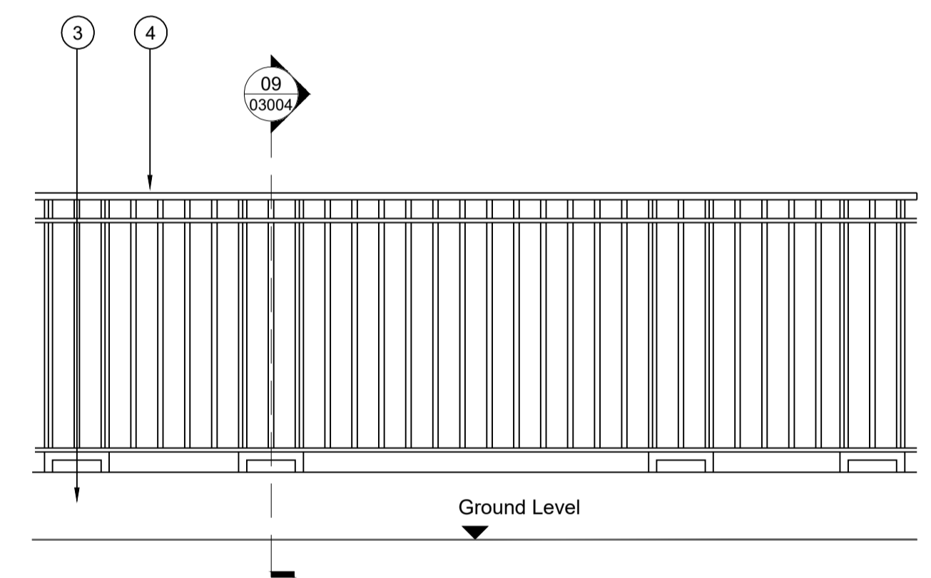
08 03004 W2a - Proposed Retaining Walls with 1.1m High Balustrade and Metal Cladding Elevation Scale 1: 20 @A1
