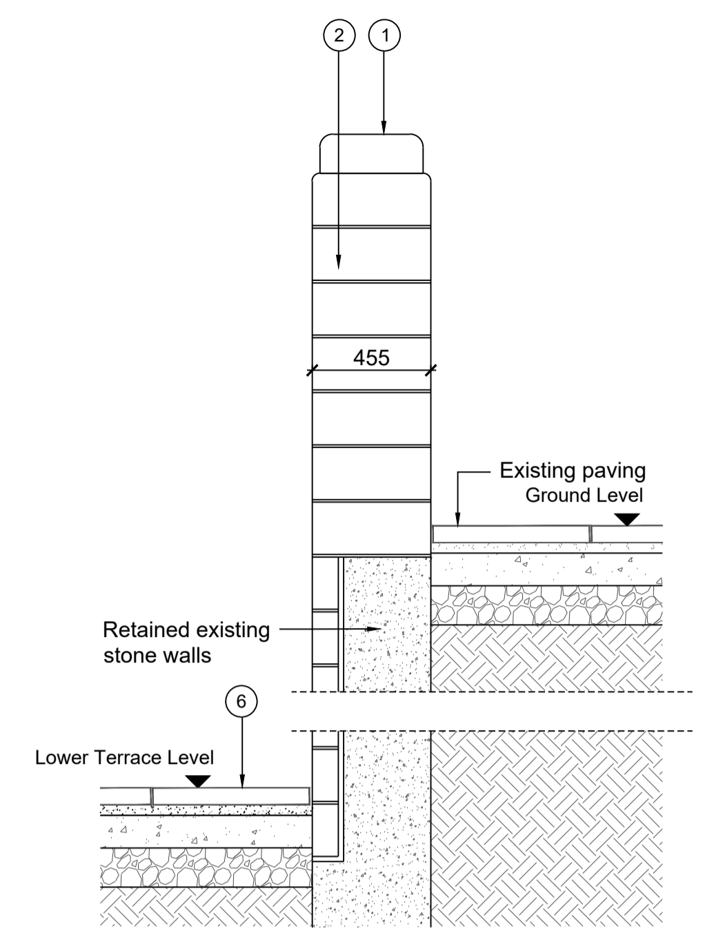
07 03004 W1a/b - Replicated Square Pier Section Scale 1: 20 @A1
