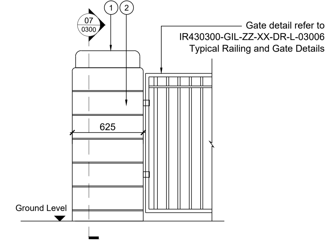
06 03004 W1b - Replicated Rectangular Pier Elevation Scale 1: 20 @A1
