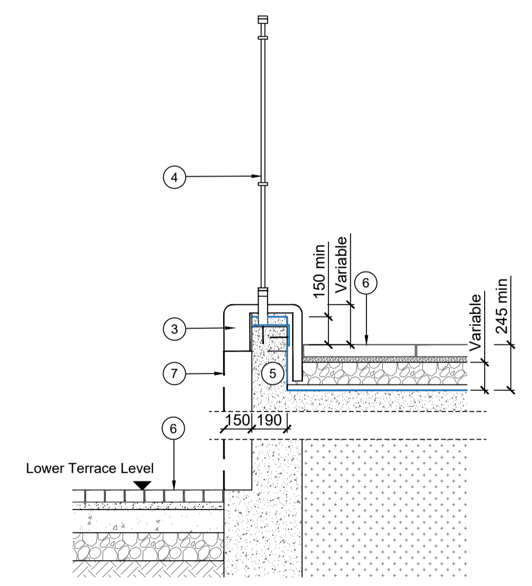
11 03004 W2c - Balustrade Section Scale 1: 20 @A1
