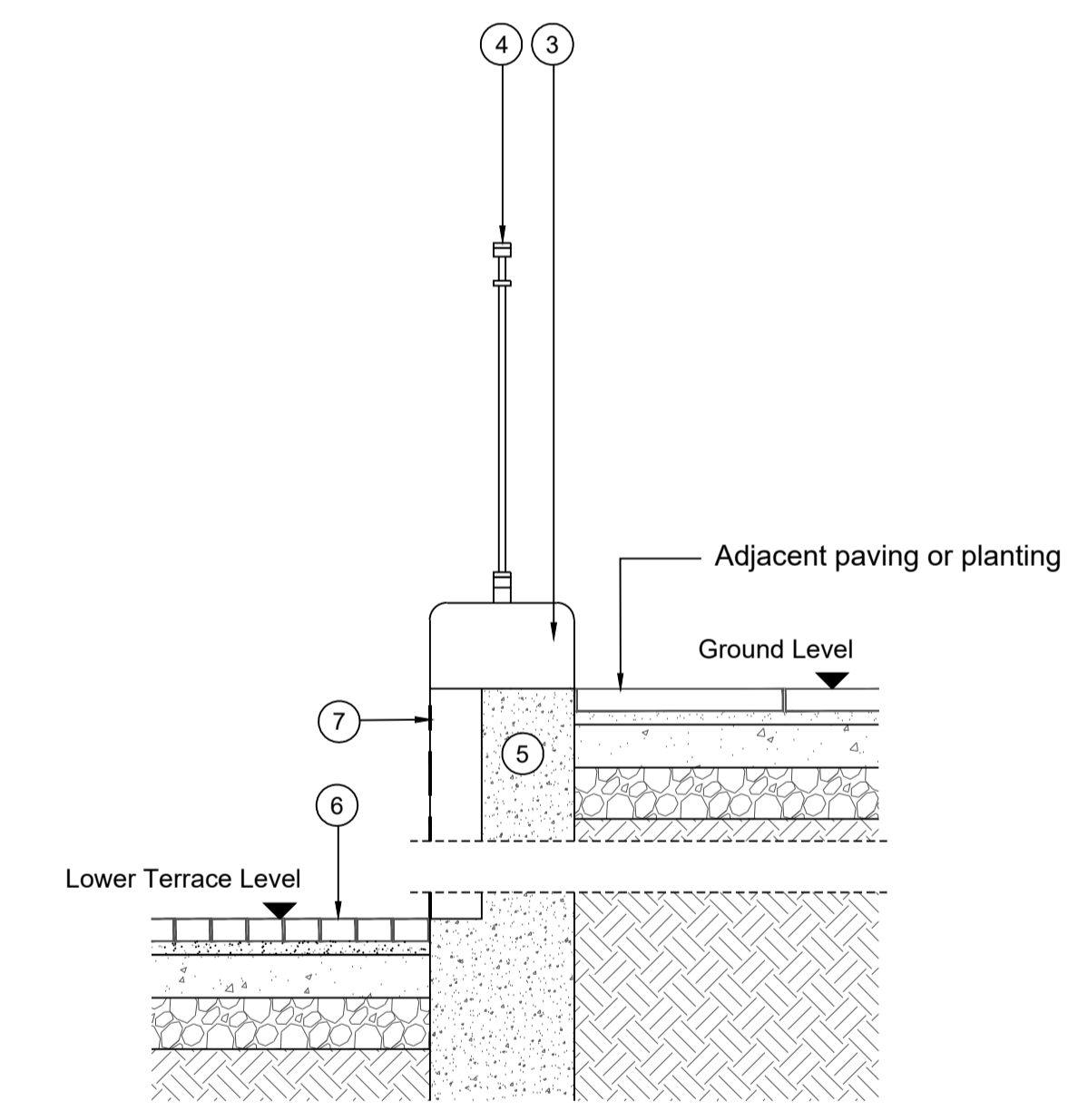
09 03004 W2a - Balustrade Section Scale 1: 20 @A1
