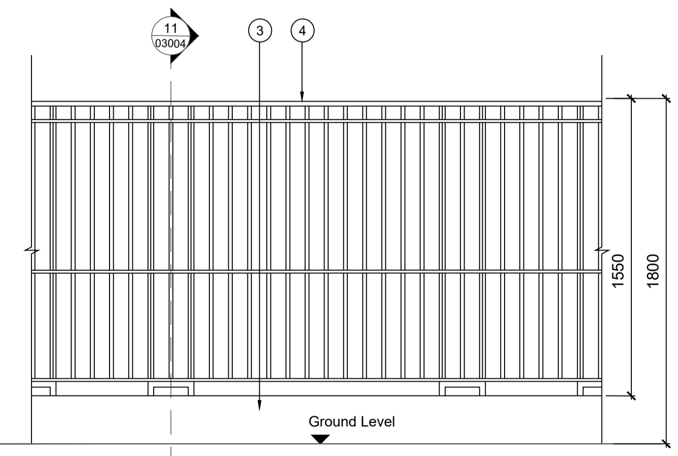
10 03004 W2c - Proposed Retaining Walls with 1.8m High Balustrade and Metal Cladding Elevation Scale 1: 20 @A1
