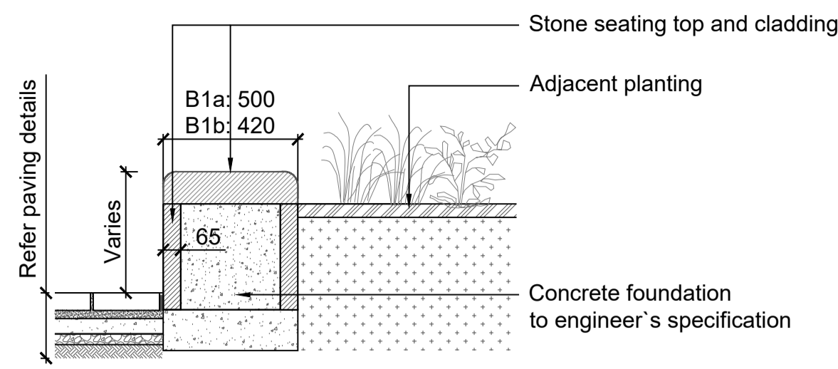
01 03004 B1a/b - Proposed Low Seating Walls Scale 1: 20 @A1
