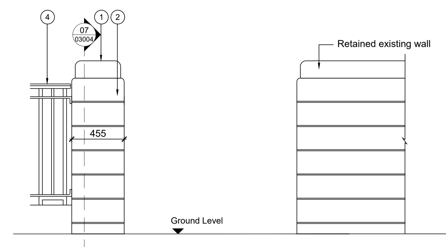
05 03004 W1a - Replicated Square Pier Elevation Scale 1: 20 @A1
