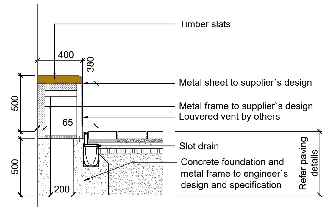
04 03004 B3b - Proposed Low Seating Walls with Timber Slat & Louvered Panels Scale 1: 20 @A1
