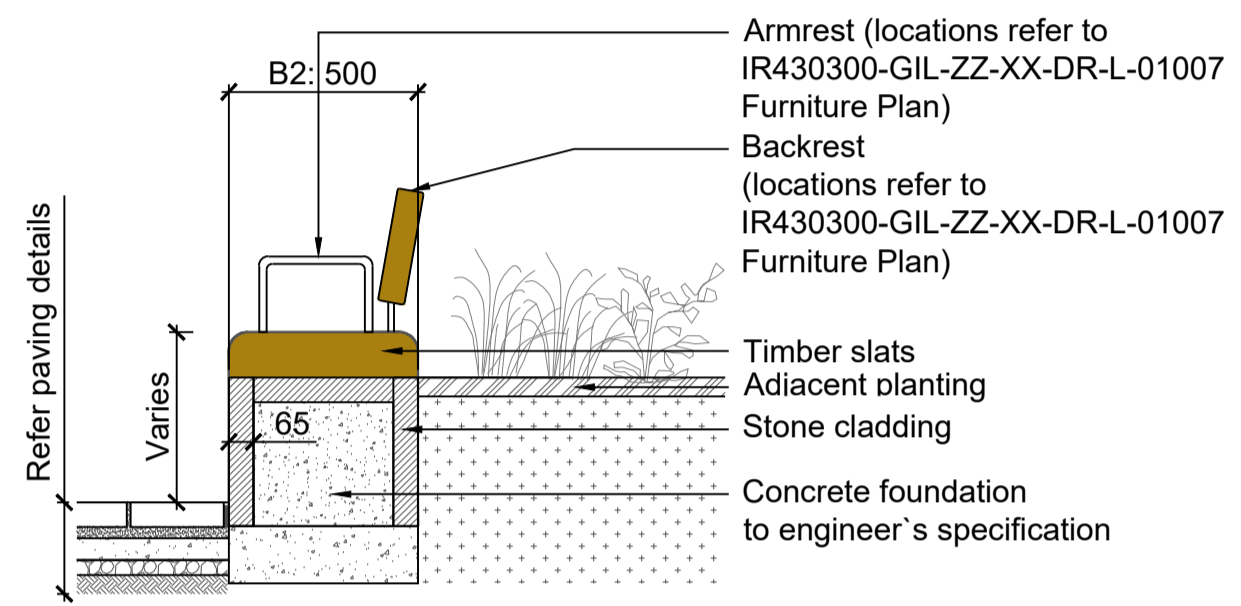
02 03004 B2a/b - Proposed Low Seating Walls with Timber Slats Seating Scale 1: 20 @A1
