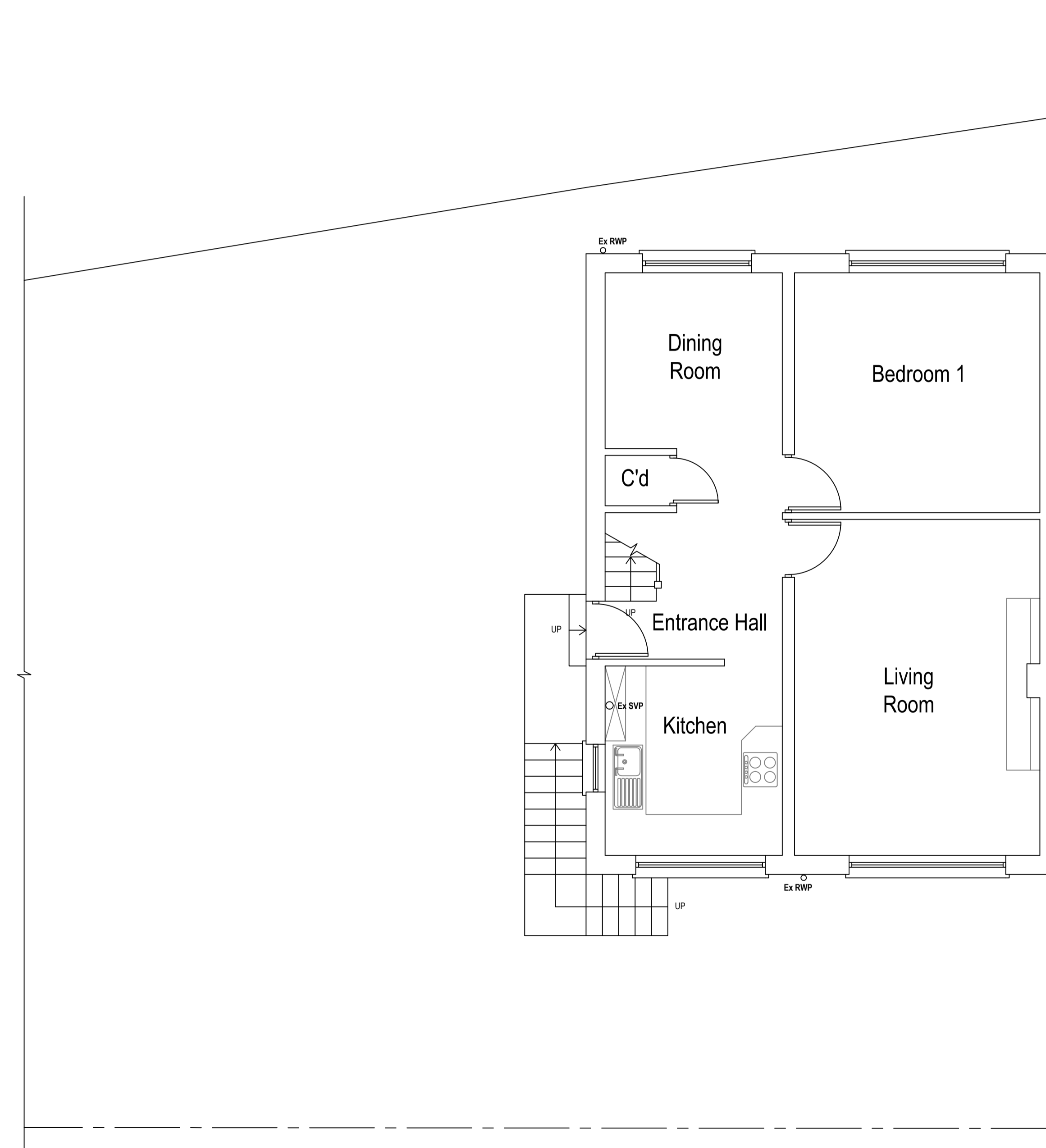
Existing First Floor Plan Area ca. 54.55 m 2
