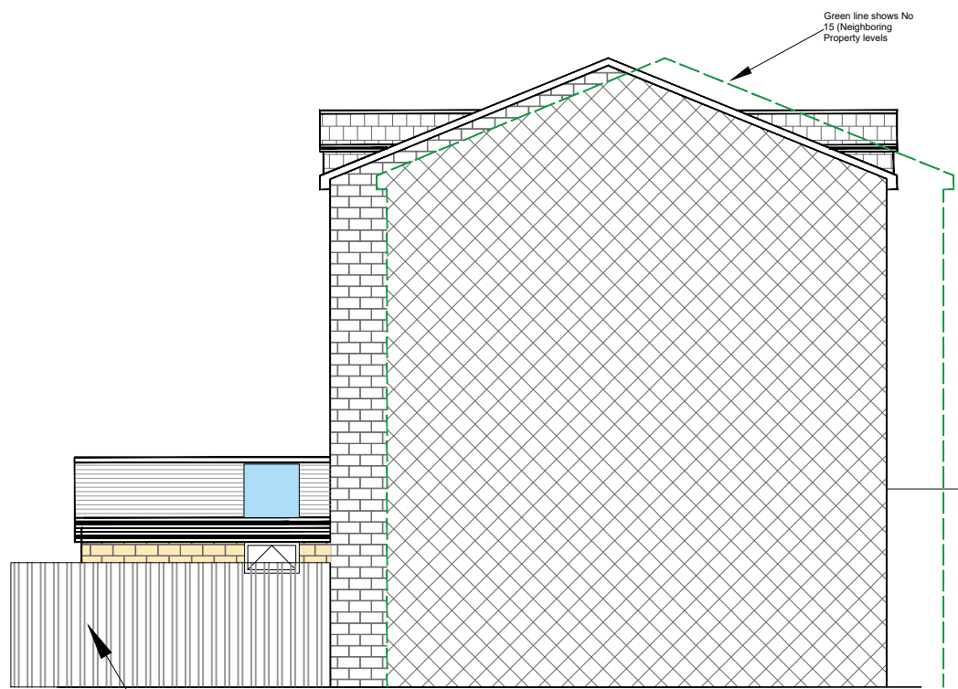
PROPOSED SIDE ELEVATION (South West)
