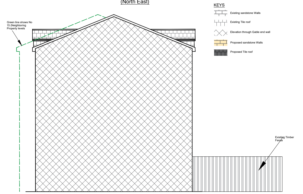
EXISTING SIDE ELEVATION (North East)
