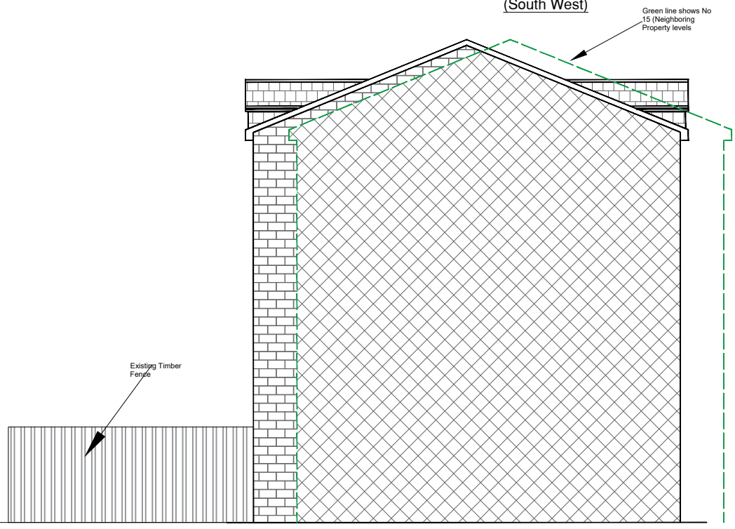
EXISTING SIDE ELEVATION (South West)
