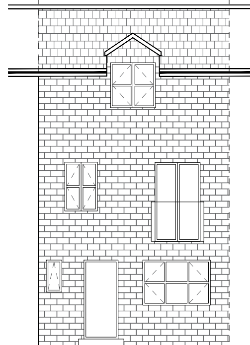
EXISTING FRONT ELEVATION (North West)
