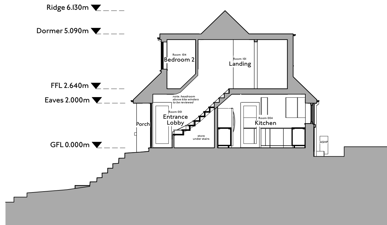
1 1:100 Proposed Section A_A
