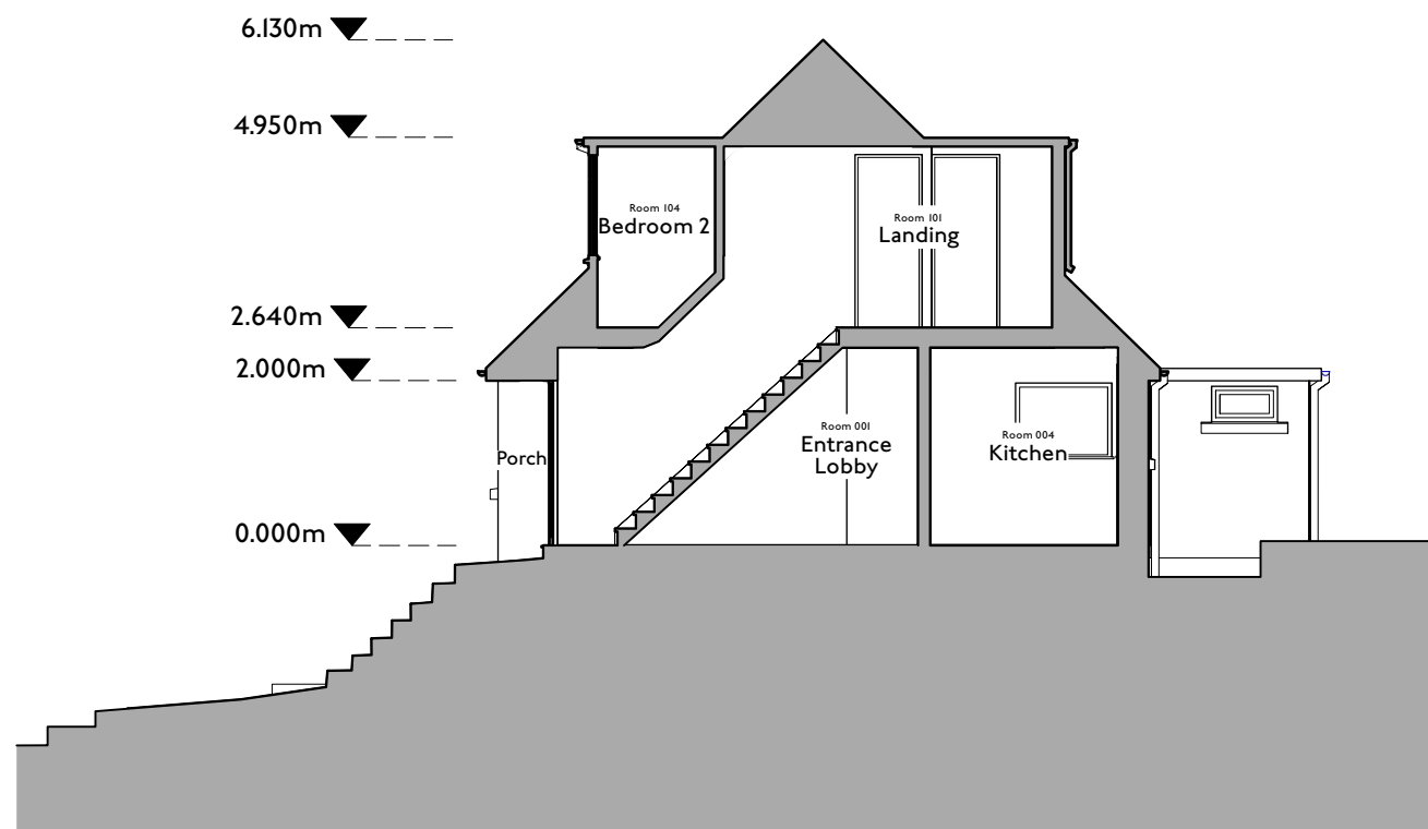
1 | 1:100 Existing Section A_A
