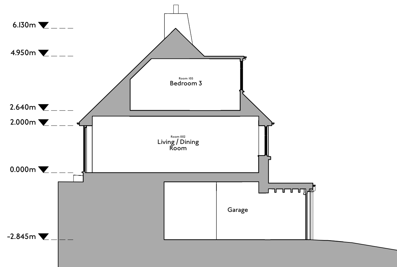
2 | 1:100 Existing Section B_B
