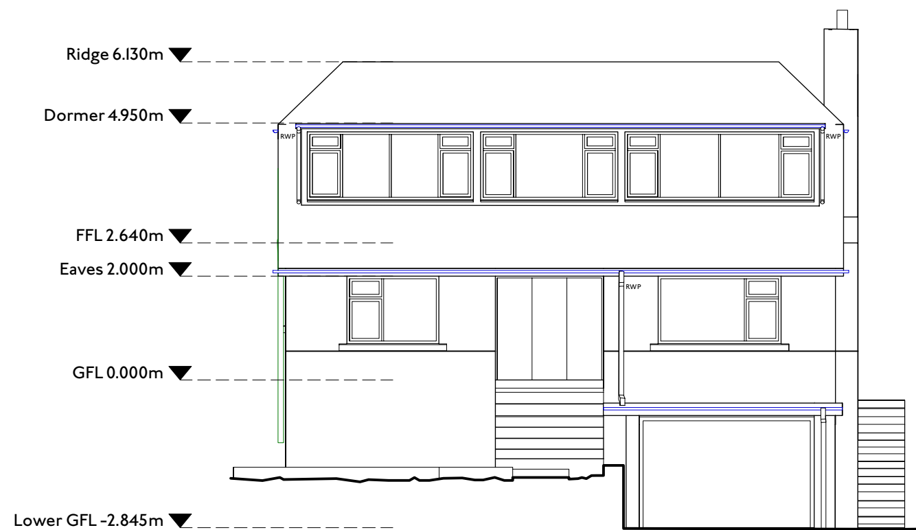
1 | 1:100 Existing Front Elevation
