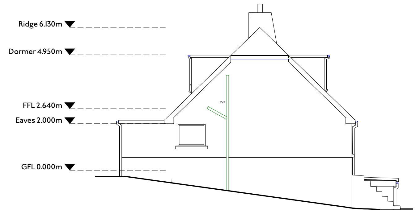
4 | 1:100 Existing Side Elevation 2
