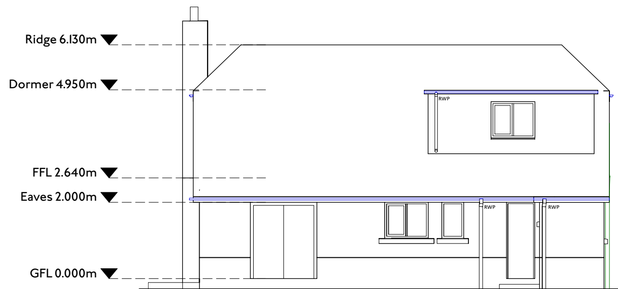
1 | 1:100 Existing Front Elevation
