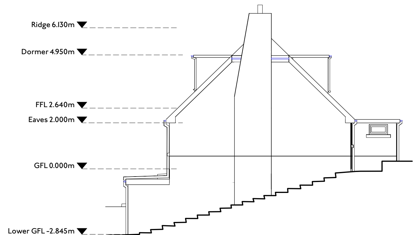
2 | 1:100 Existing Side Elevation 1
