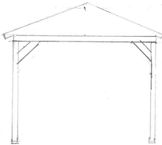
SIDE ELEVATION GARDEN SIDE
