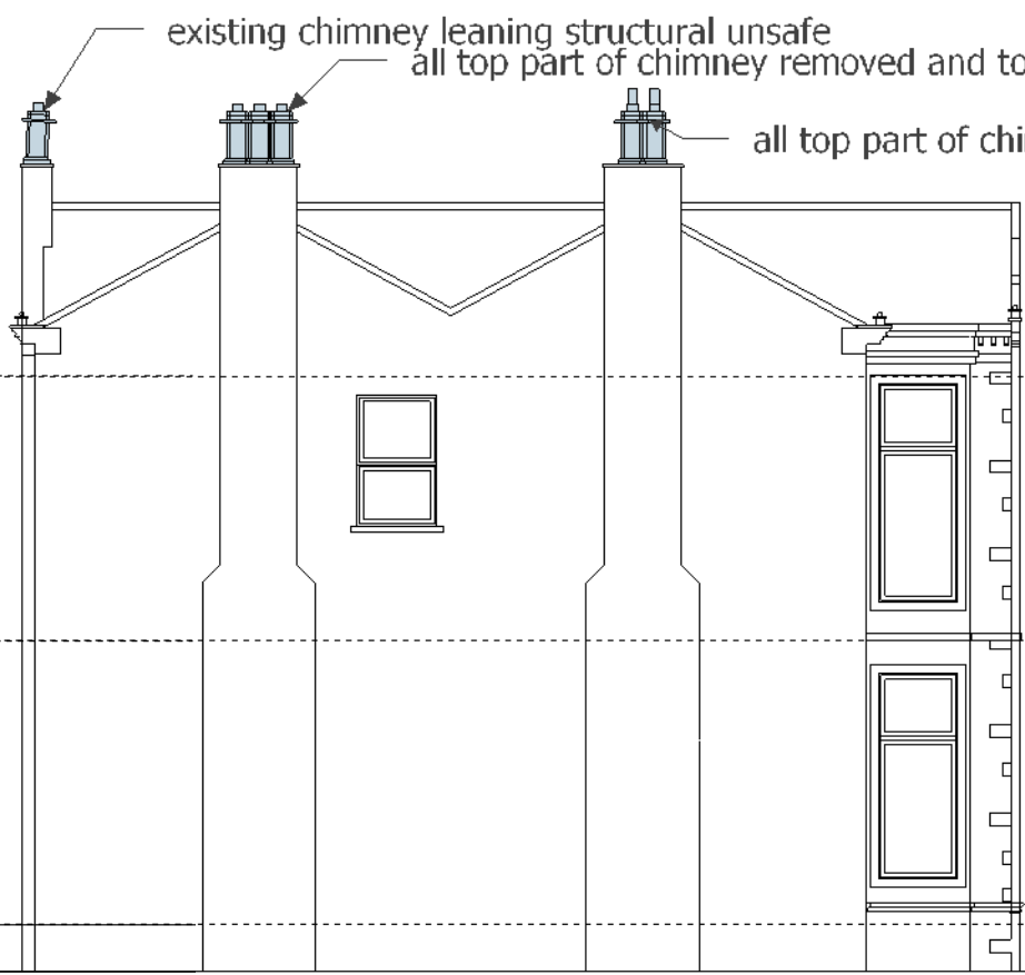
existing rear elevation north west elevation
