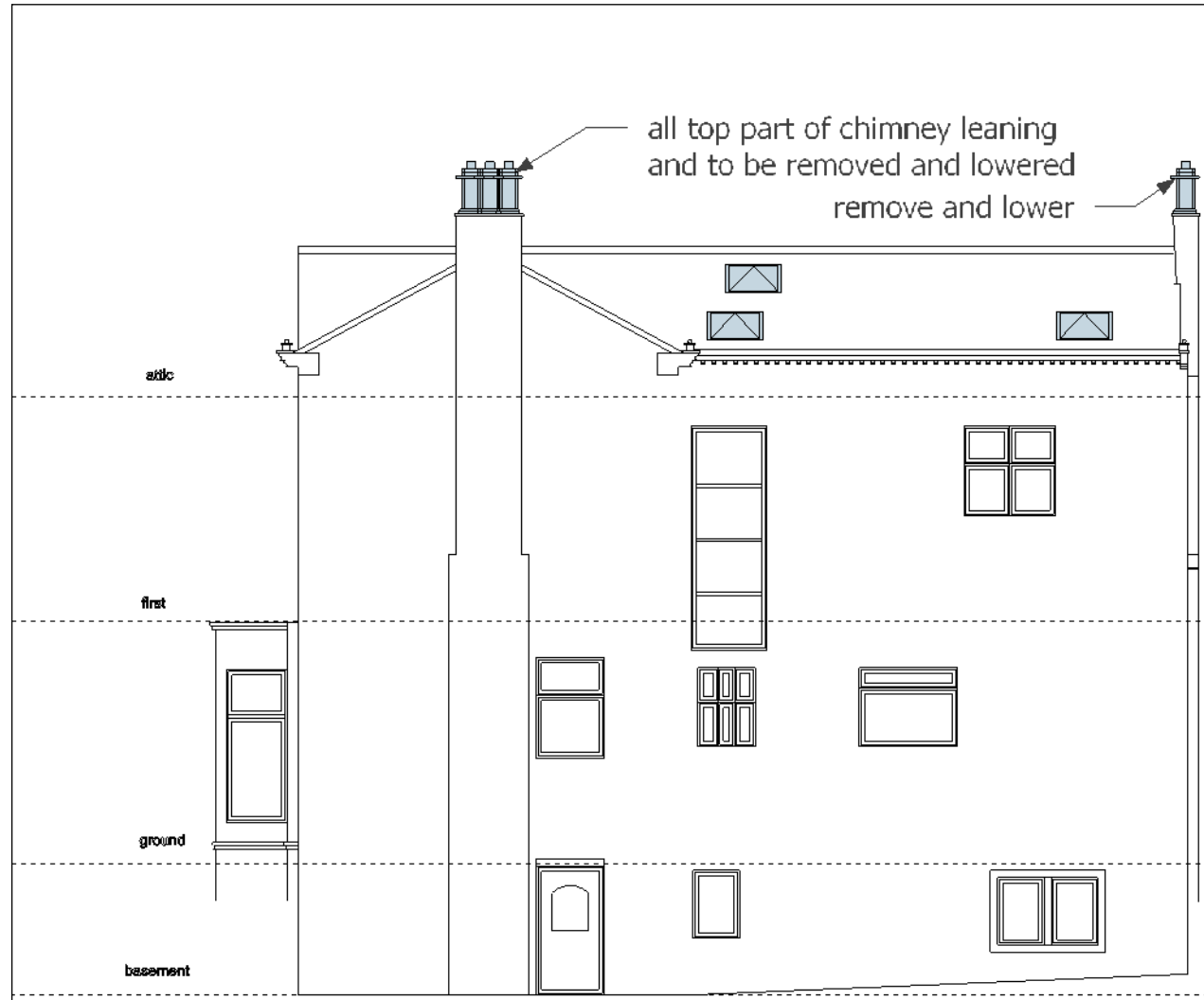
(north east elevation) existing side elevation
