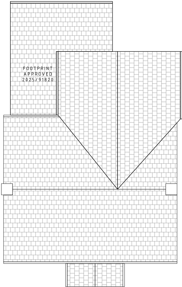
PROPOSED ROOF FLOOR PLAN
