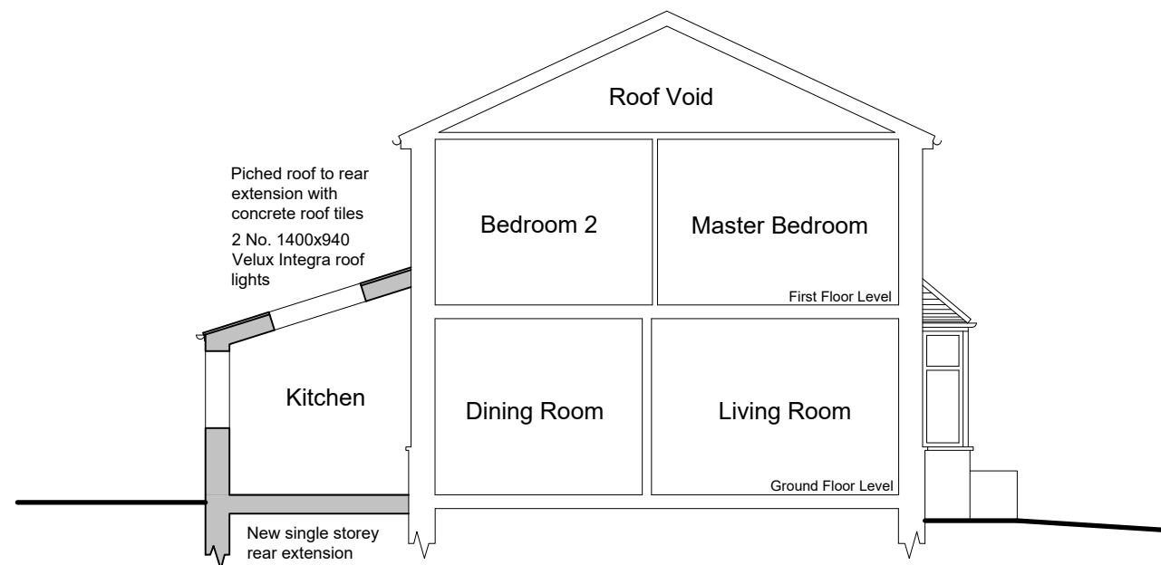
North Sectional Party Wall Elevation
