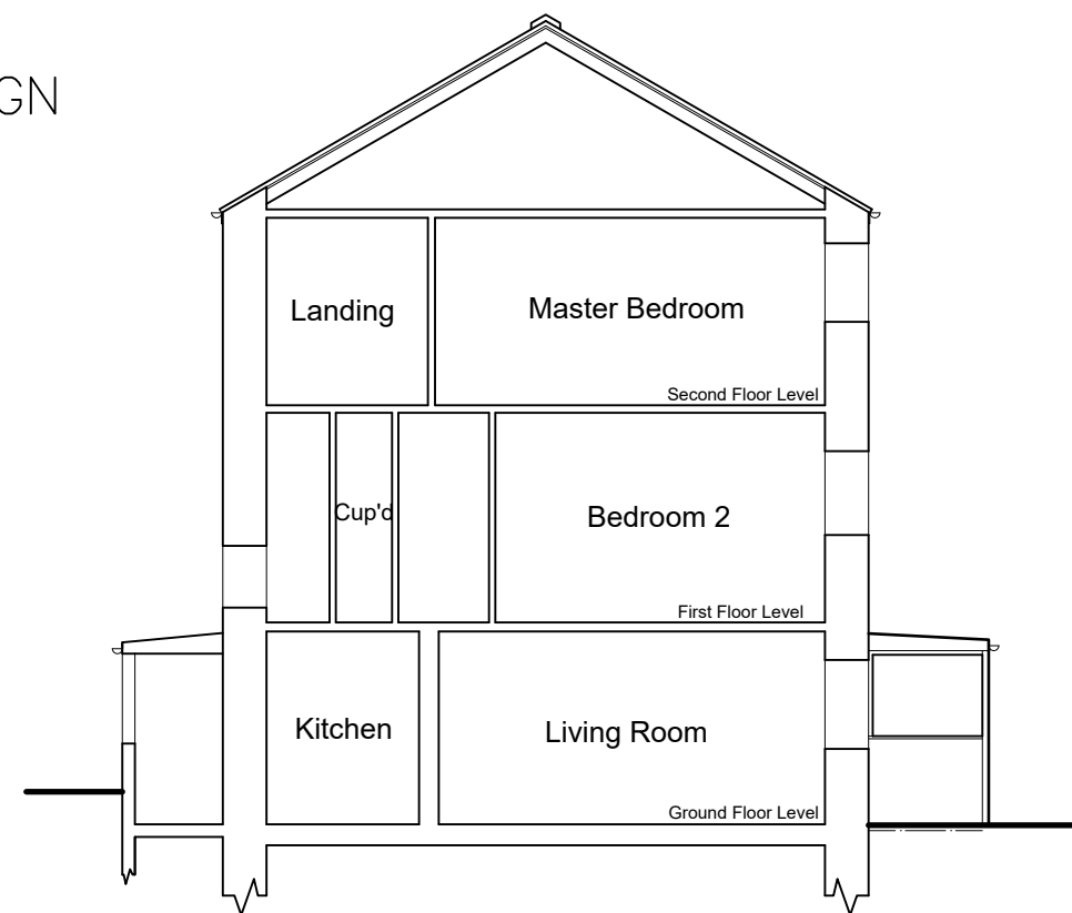
North Sectional (Party Wall) Elevation (side)
