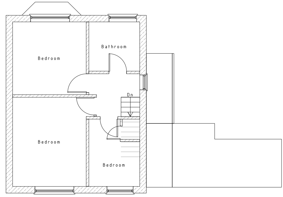
EXISTING FF PLAN
