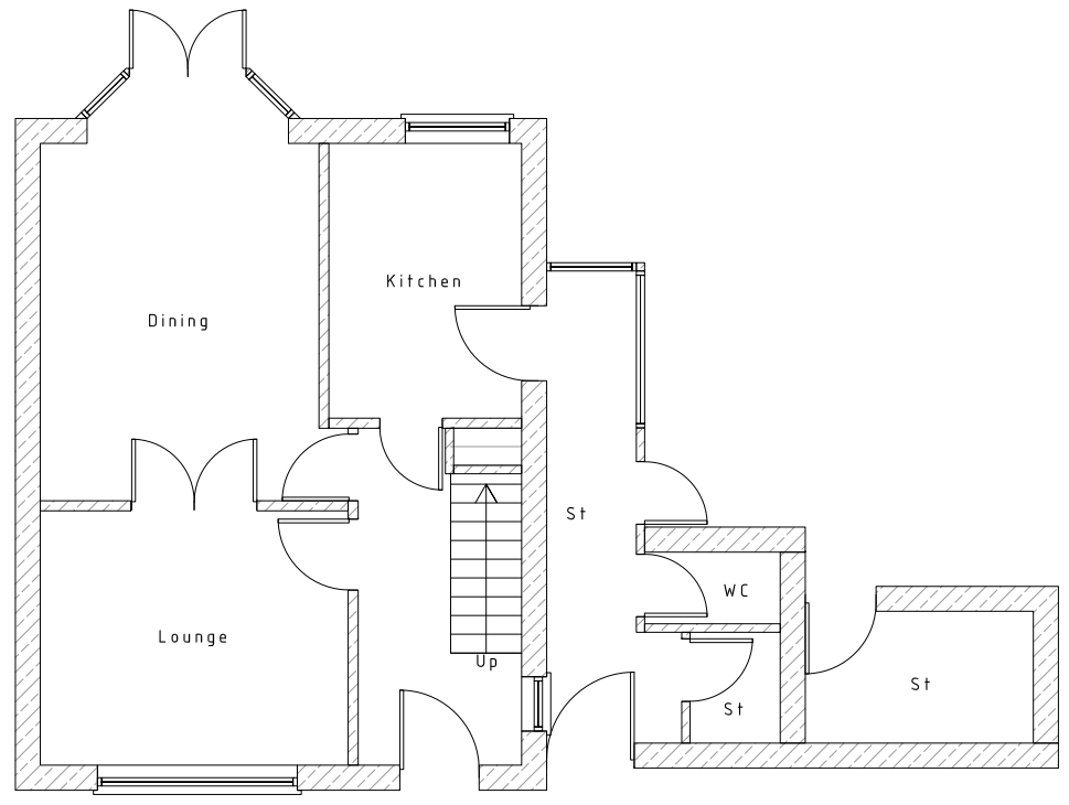
EXISTING GF PLAN
