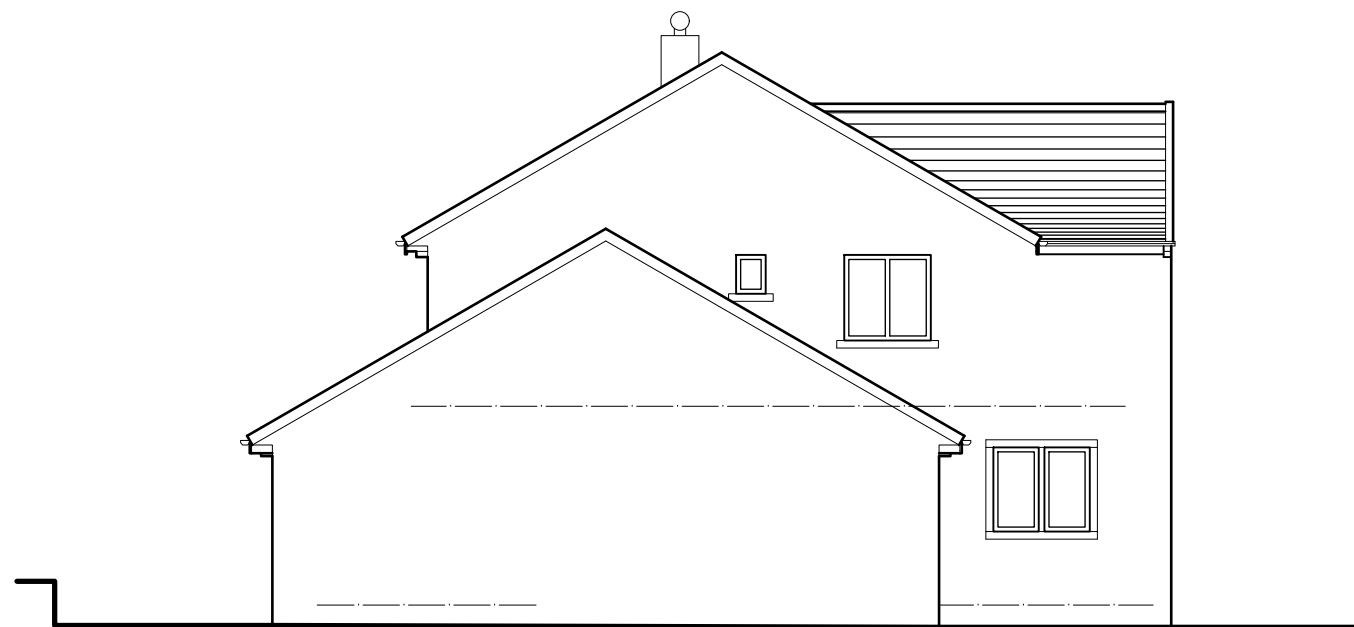
North West Elevation (side)
