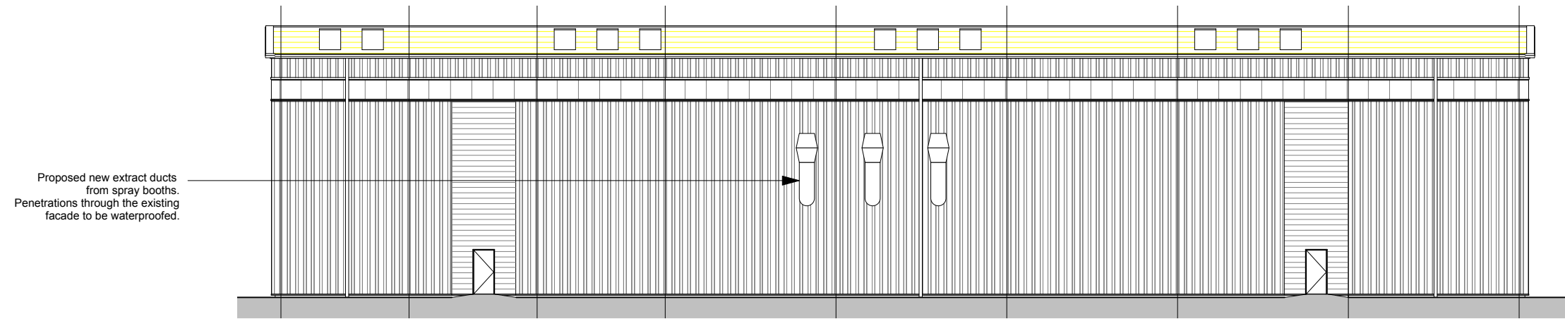
2 Proposed West Elevation Scale 1:250 @ A3
