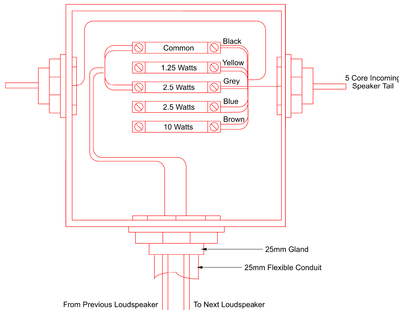
Junction Box Typical PA Connections Daisy Chained
