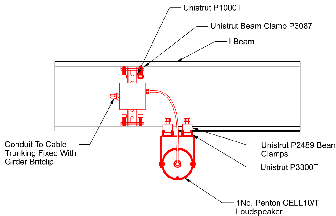
Canopy Girder Mounted Loudspeaker Detail
