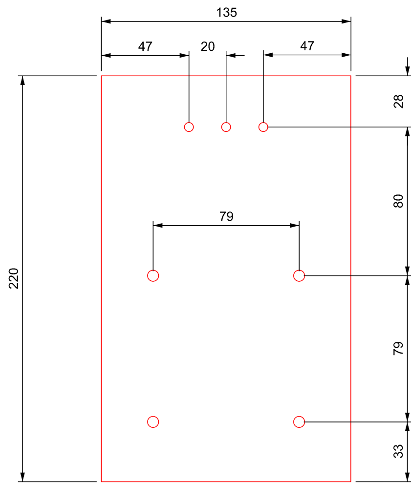
Plate A Detail for PA Loudspeaker & Junction Box
