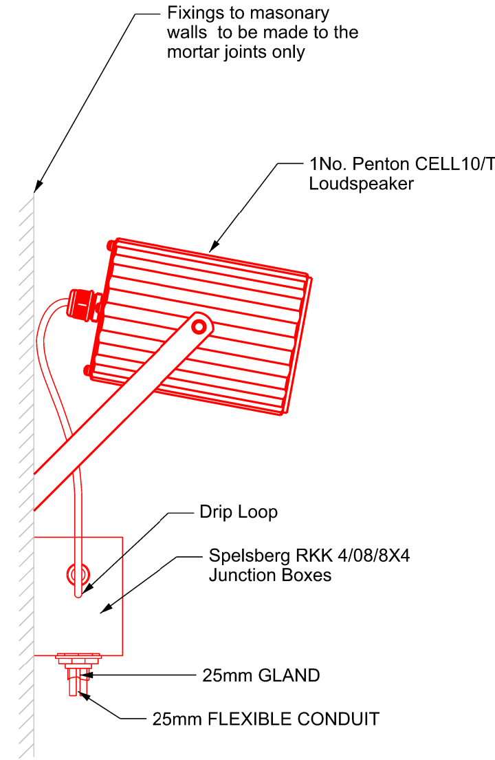
Wall Mounted Loudspeaker Detail
