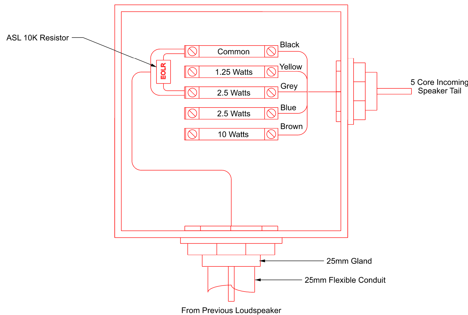
Junction Box Typical PA Connections End of Line
