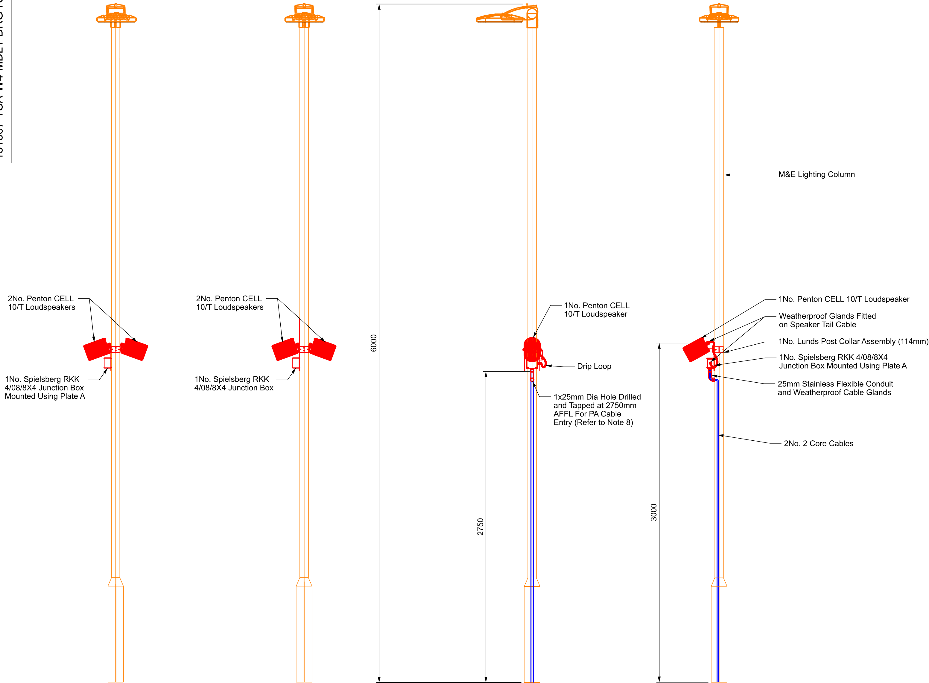
Lighting Column Mounted Speakers
