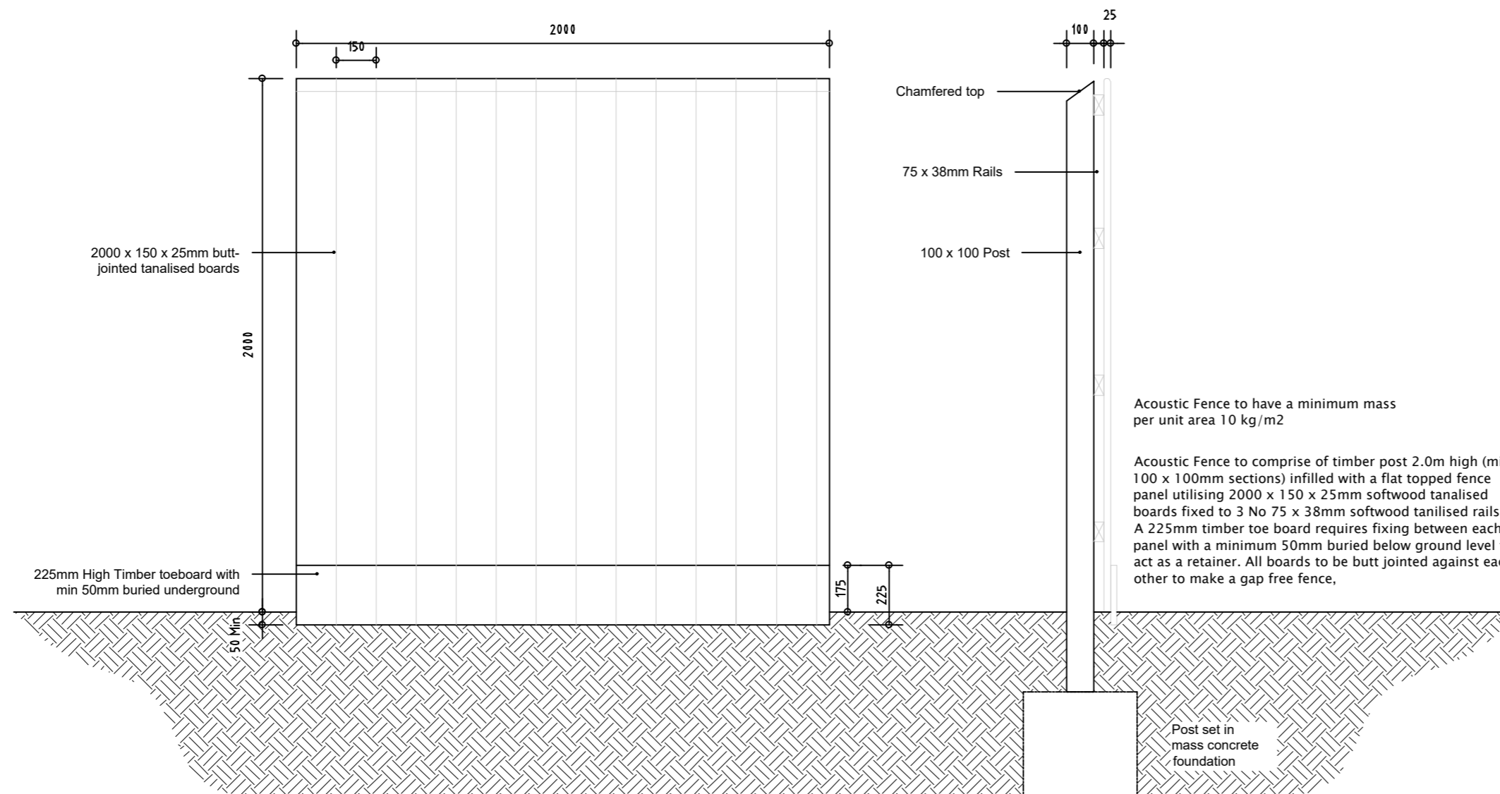
2000mm SOLID ACOUSTIC TIMBER FENCE
