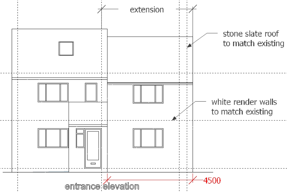
entrance elevation
