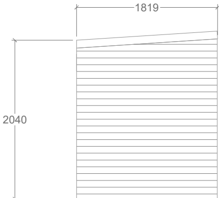
SHED 2 - SIDE
