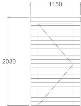
SHED 1 - FRONT
