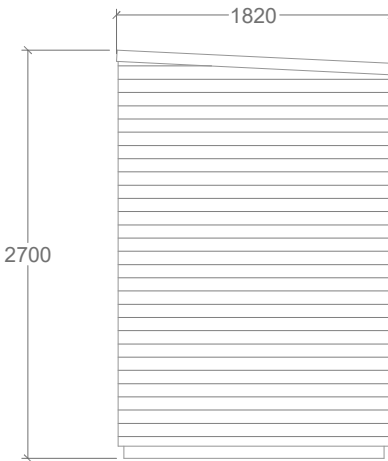
WC - SIDE
