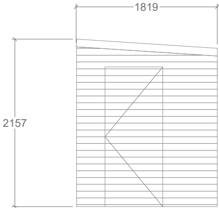
SHED 2 - SIDE
