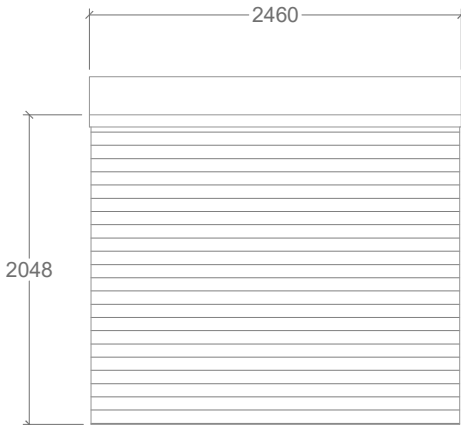
CHANGING CUBICLE - BACK
