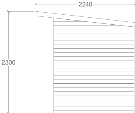
CHANGING CUBICLE - SIDE
