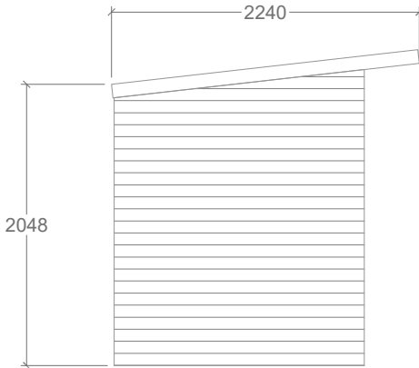
CHANGING CUBICLE - SIDE
