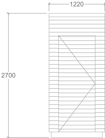
WC - FRONT
