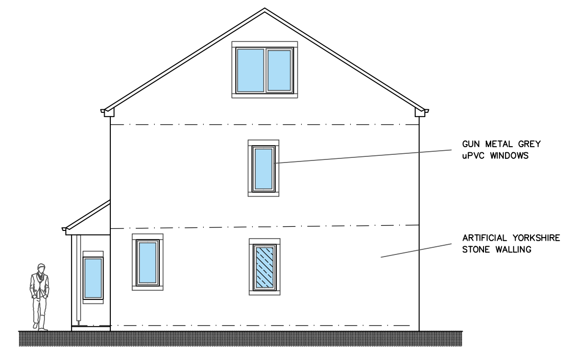
NORTH-WEST ELEVATION (LOWER)
