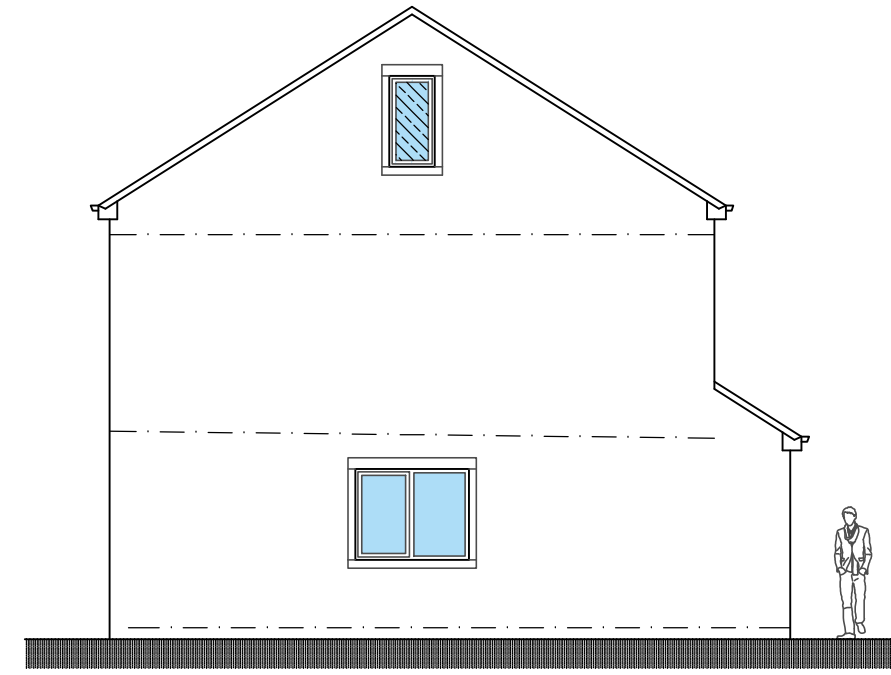
SOUTH-EAST ELEVATION (UPPER)
