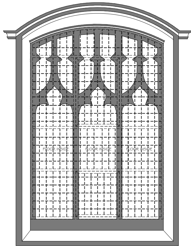
THREE ARCHES - BIG WINDOW SECTIONAL & ELEVATION DETAILS
