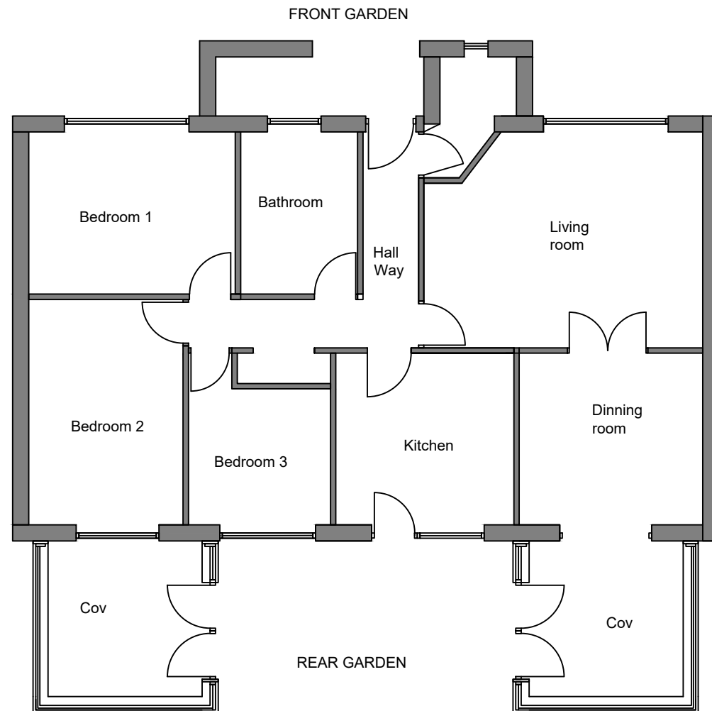
EXISTING GROUND FLOOR PLANS
