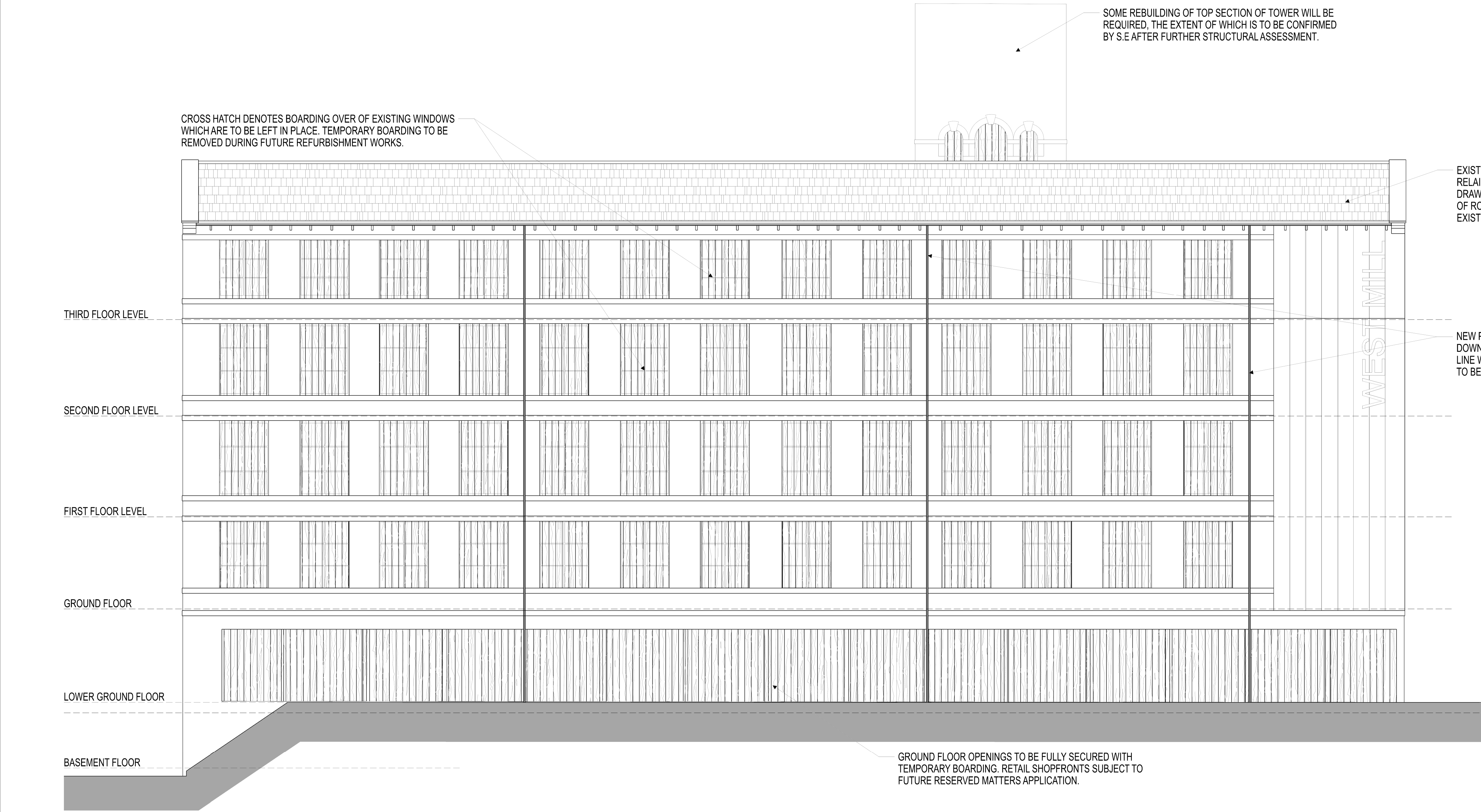
ELEVATION C
