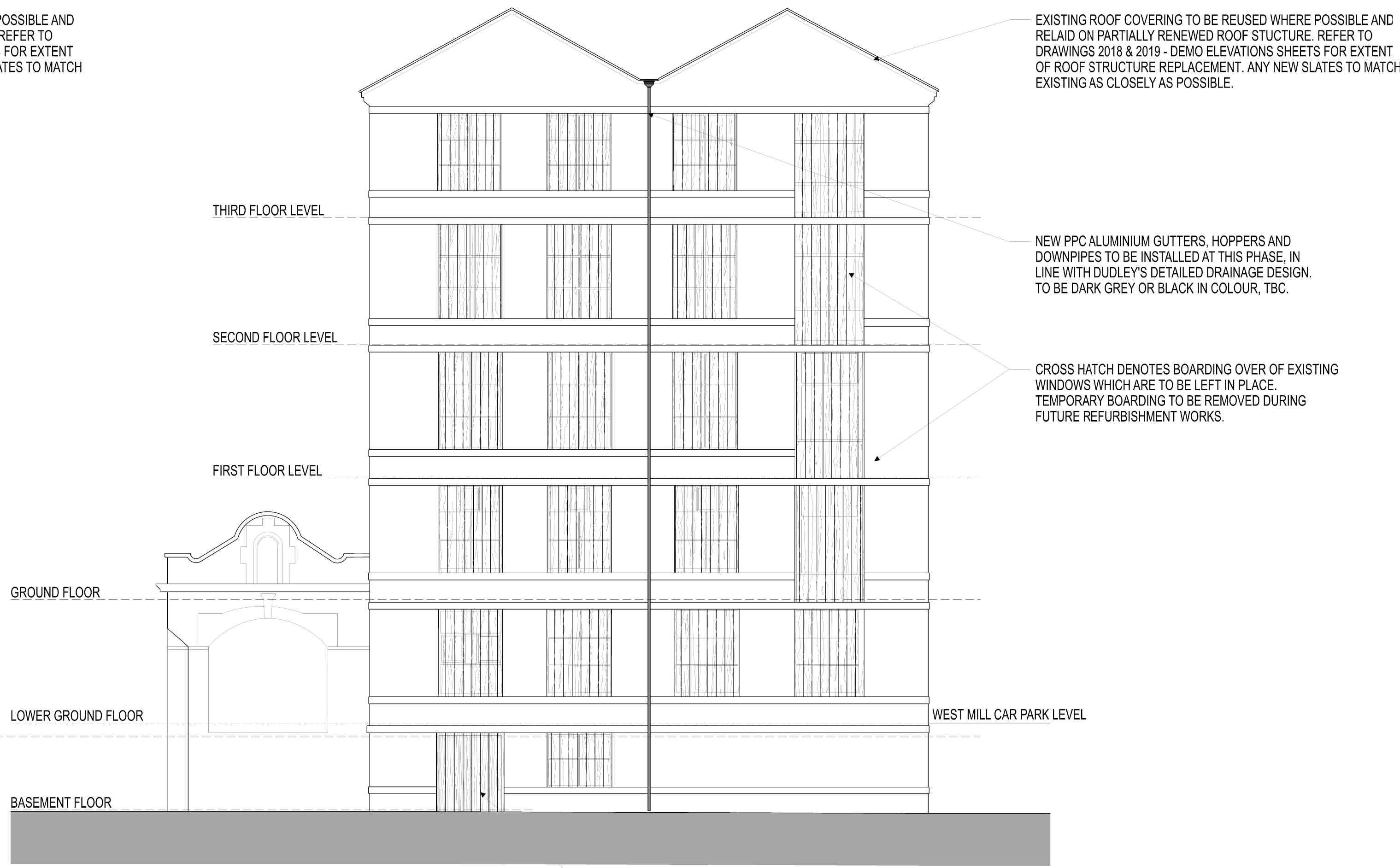
ELEVATION D
