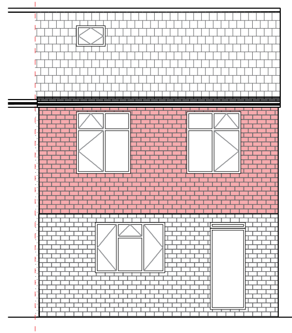
PROPOSED REAR ELEVATION (West)
