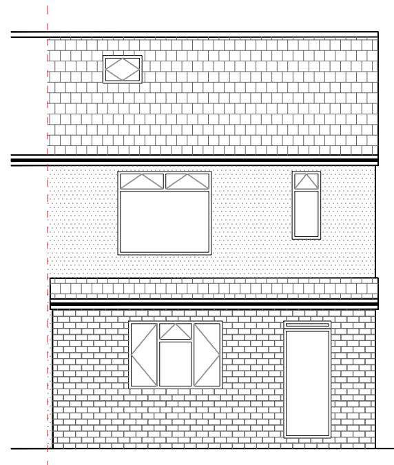
EXISTING REAR ELEVATION (West)
