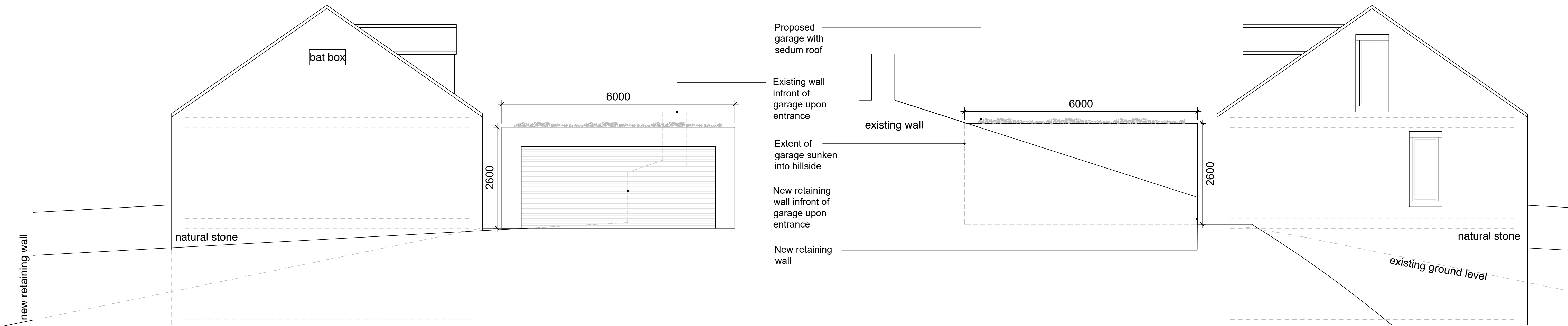
Proposed Elevation A Scale 1:50
