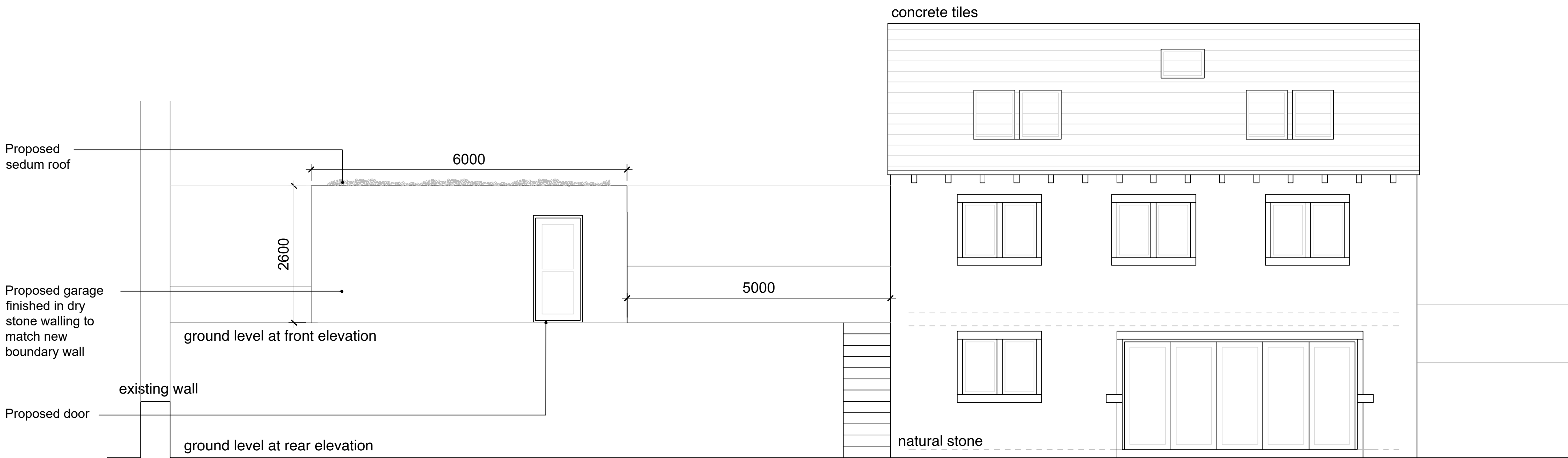
Proposed Elevation C Scale 1:50
