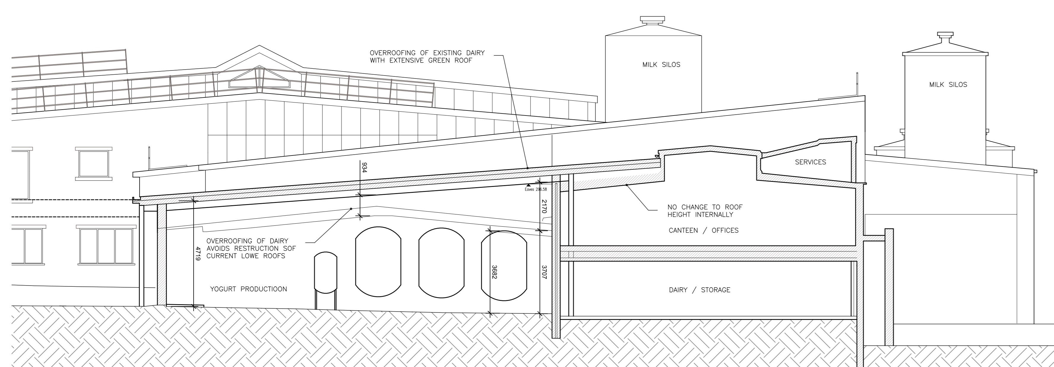
CROSS SECTION DD - LOOKING SOUTH (OVER ROOFING OF YOGURT DEPT)
