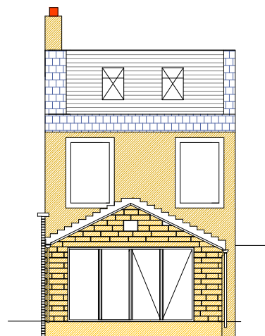
North Elevation
