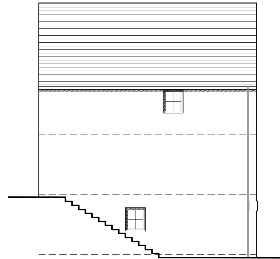
SIDE ELEVATION
