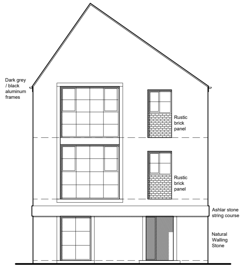
FRONT ELEVATION
