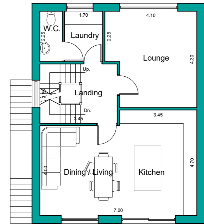
UPPER GROUND FLOOR PLAN
