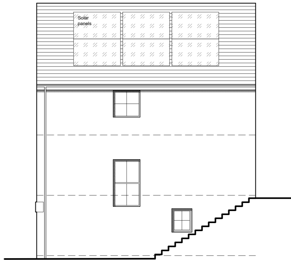
SIDE ELEVATION
