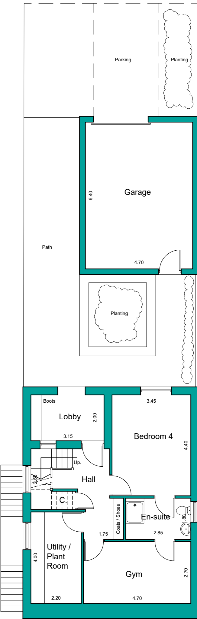
LOWER GROUND FLOOR PLAN TYPE A
