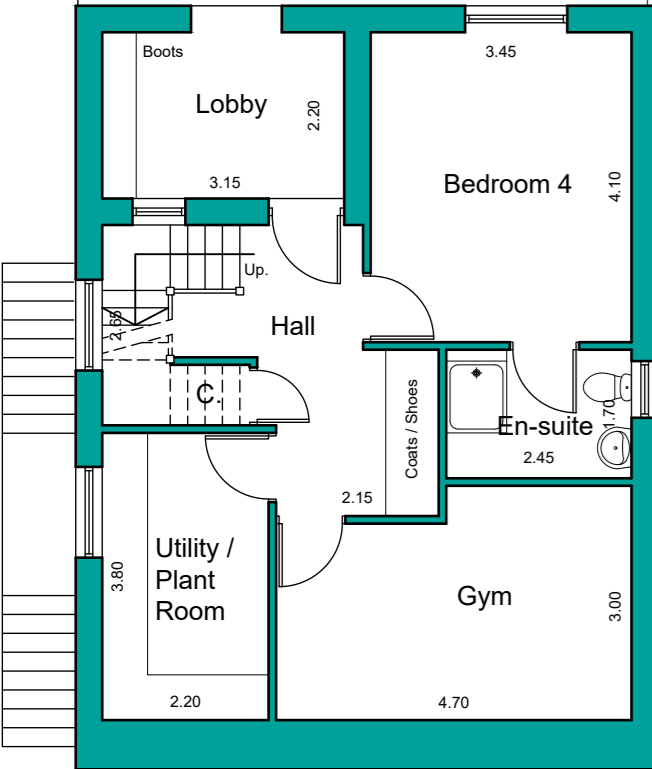
LOWER GROUND FLOOR PLAN TYPE B
