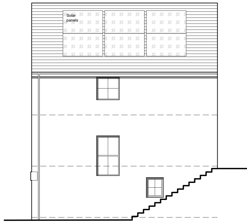
SIDE ELEVATION
