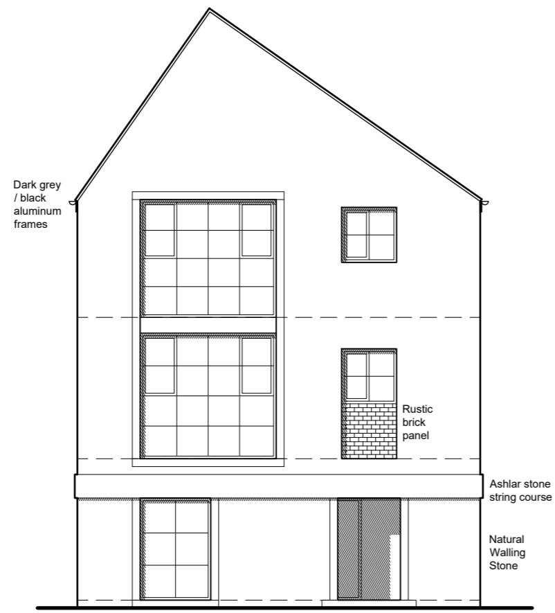
FRONT ELEVATION
