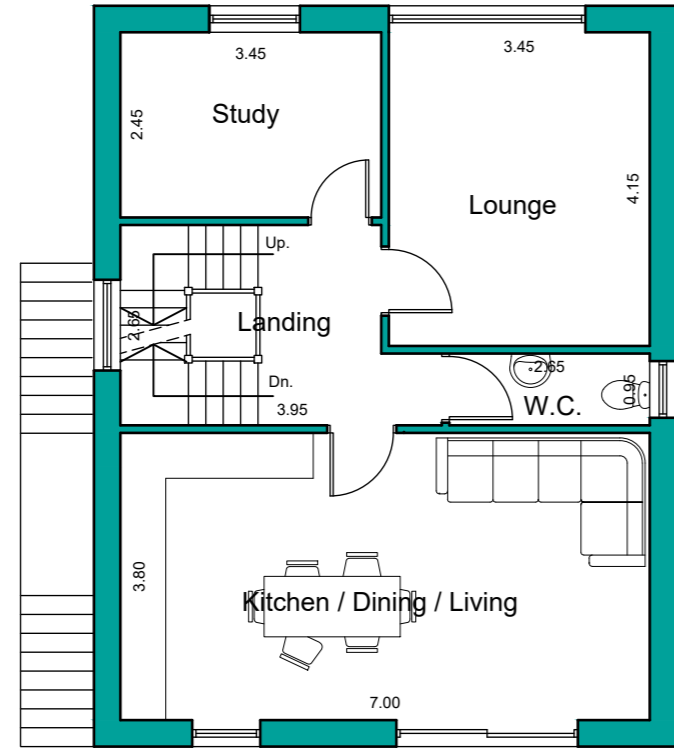
UPPER GROUND FLOOR PLAN
