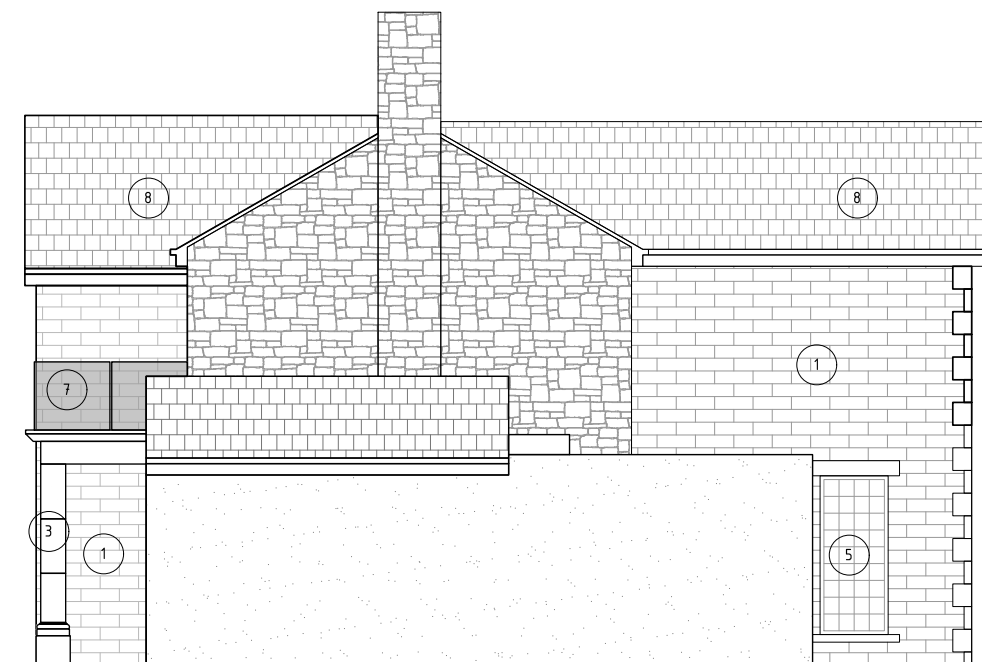
PROPOSED OTHER SIDE ELEVATION
