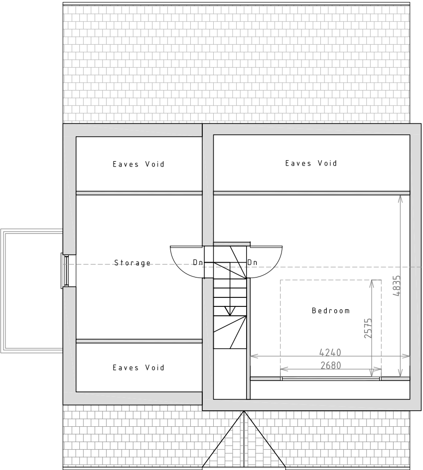
PROPOSED LOFT FLOOR PLAN
