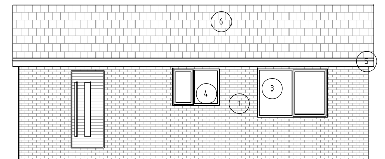
PROPOSED OUTBUILDING REAR ELEVATION
