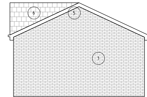
PROPOSED OUTBUILDING 0.SIDE ELEVATION
