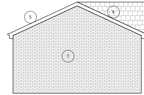
PROPOSED OUTBUILDING SIDE ELEVATION
