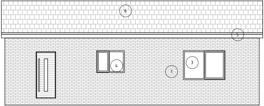
PROPOSED OUTBUILDING REAR ELEVATION
