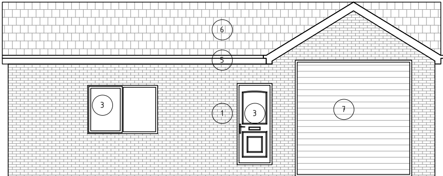
PROPOSED OUTBUILDING FRONT ELEVATION
