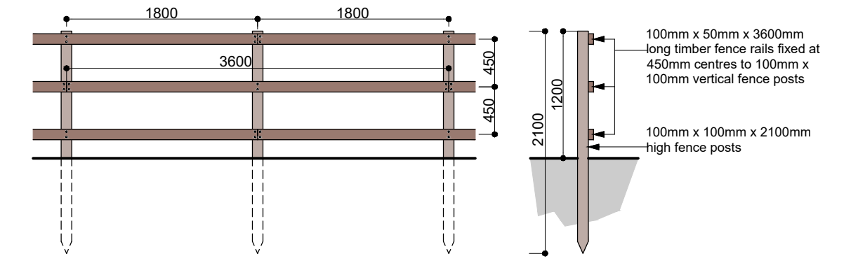
fence detail - 1:50
