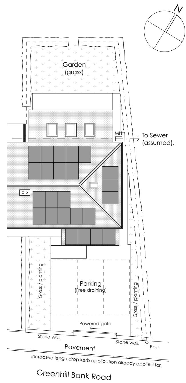
Block Plan 1:200
