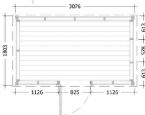
VIEW PLAN
