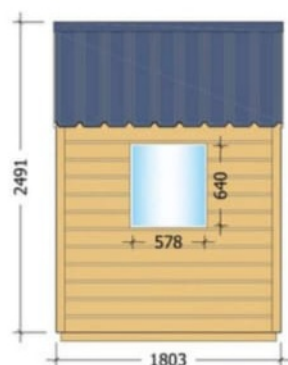
RH SIDE ELEVATION
