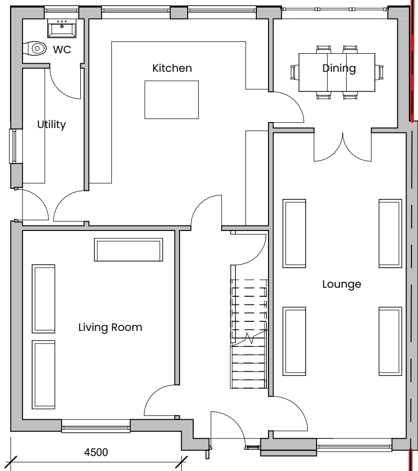
1 Proposed Ground Floor Plan 1 : 100
