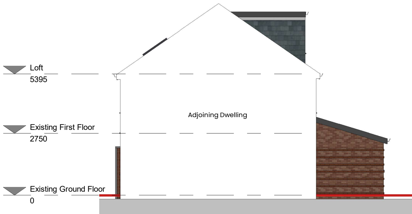
2 Proposed Adjoining Elevation 1:100
