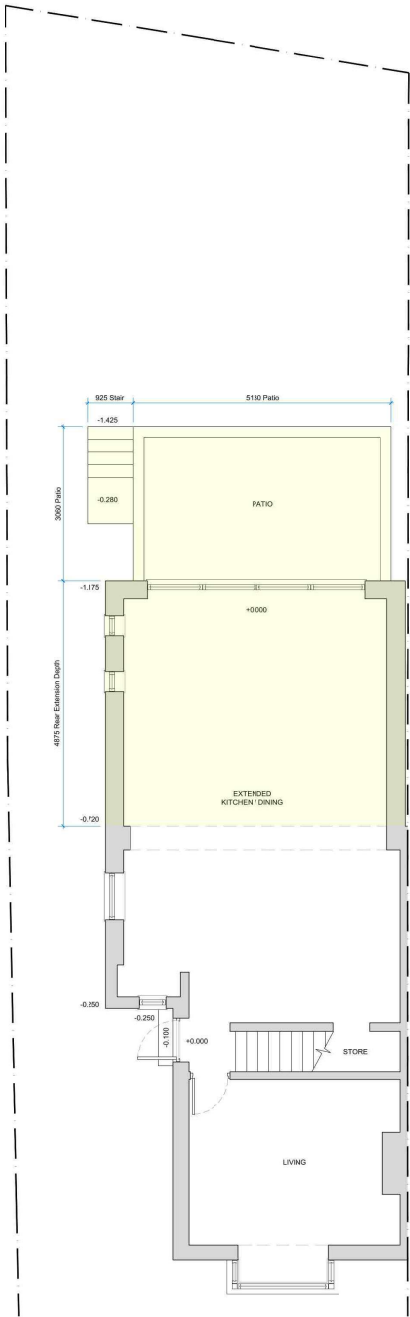
GROUND FLOOR GA PLAN / PART SITE LAYOUT EXISTING AND PROPOSED 1:50
