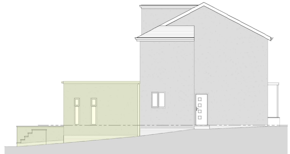
SIDE ELEVATION - EXISTING / PROPOSED 1:50
