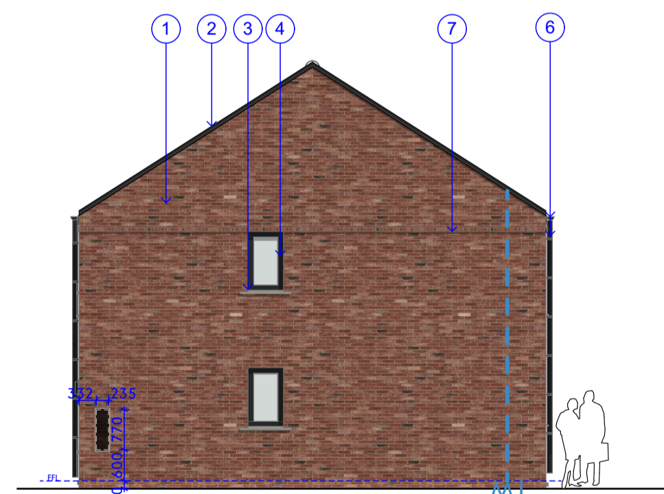
E-04 Elevation
