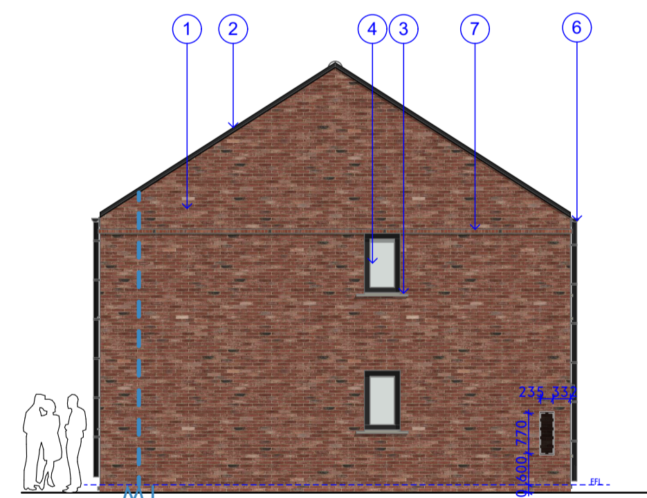
E-03 Elevation
